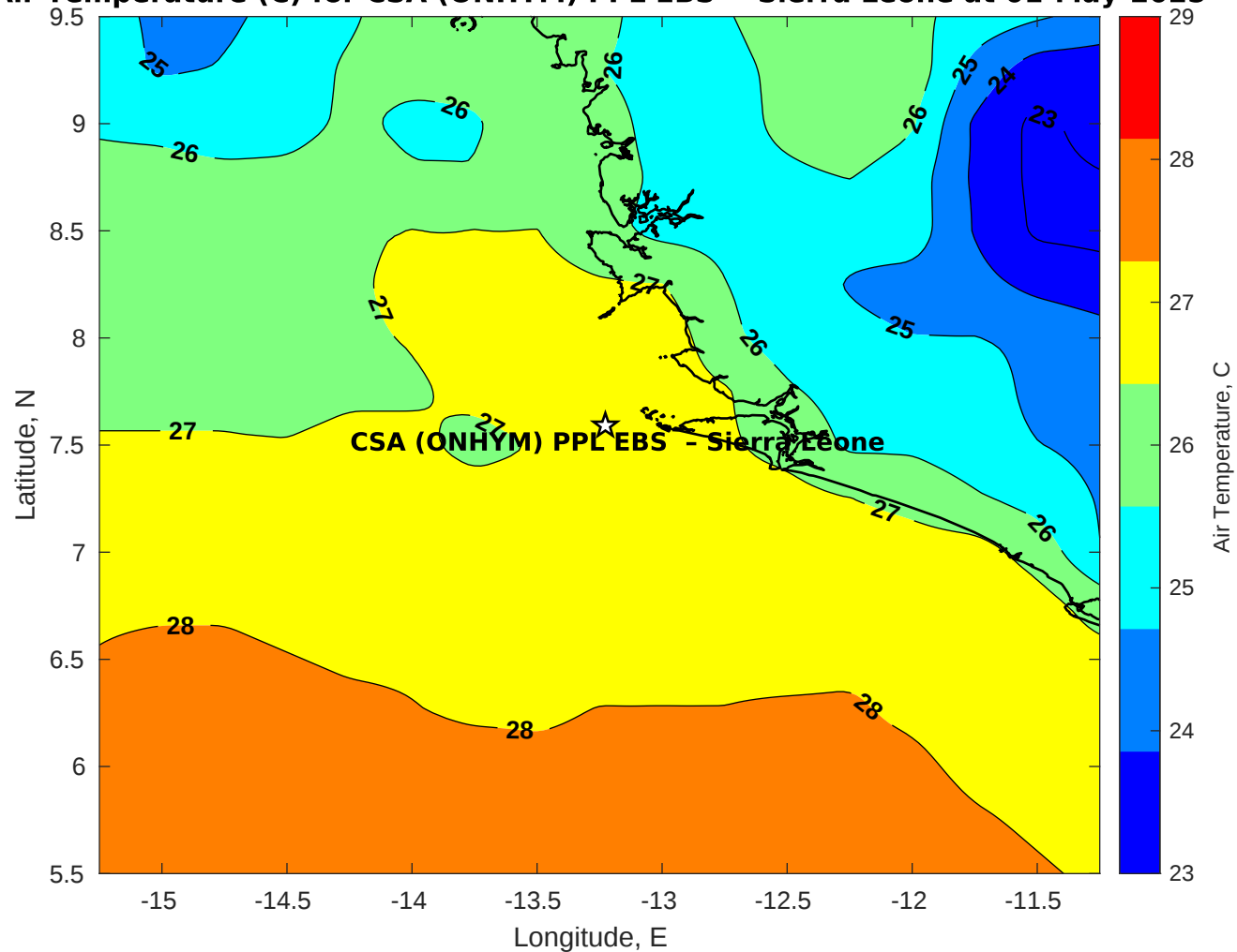
Air Temperature (C) for CSA (ONHYM) PPL EBS - Sierra Leone at 01-May-2025
