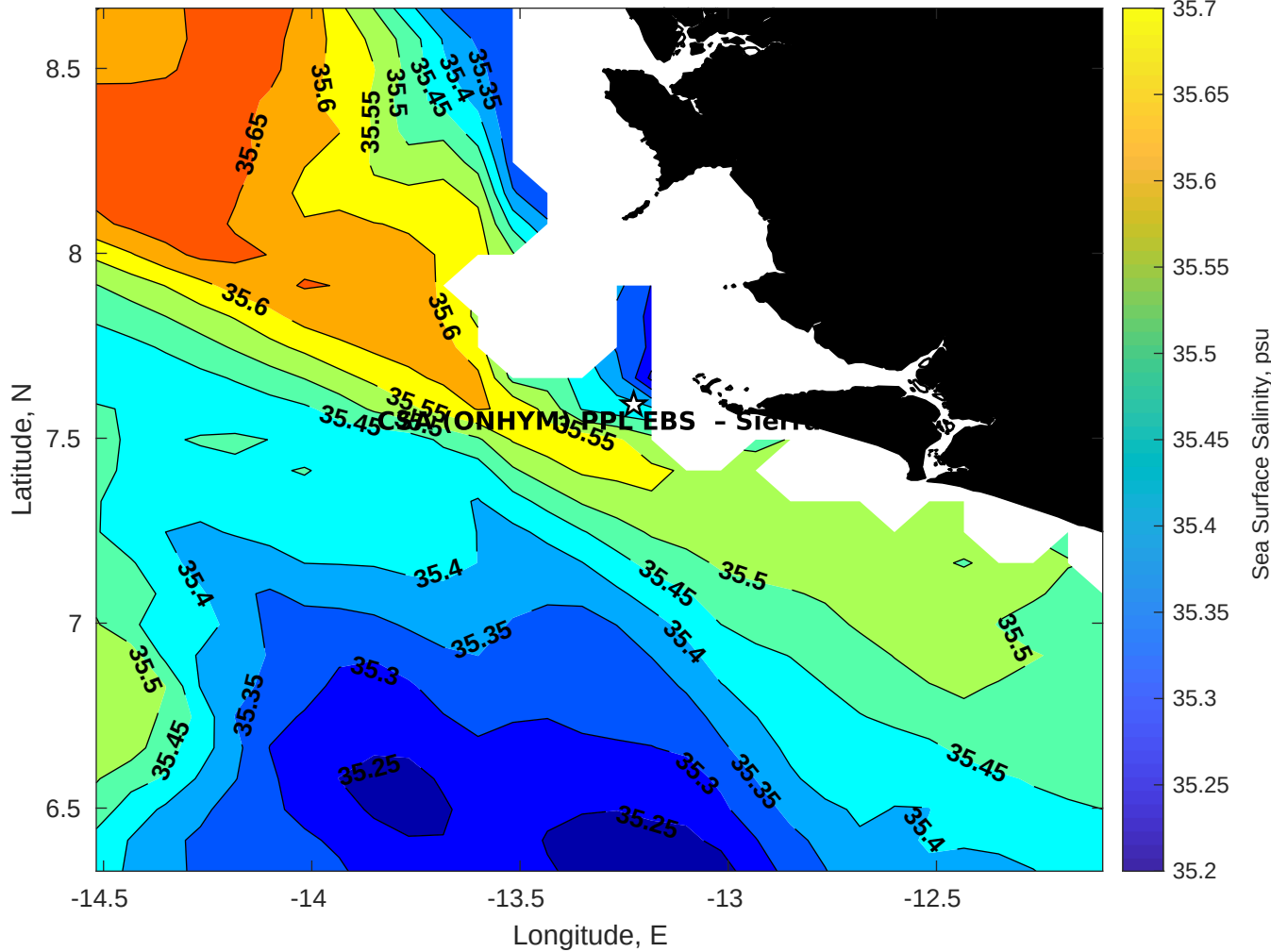
Surface Salinity for CSA (ONHYM) PPL EBS - Sierra Leone at 30-Apr-2025 00:00:00
