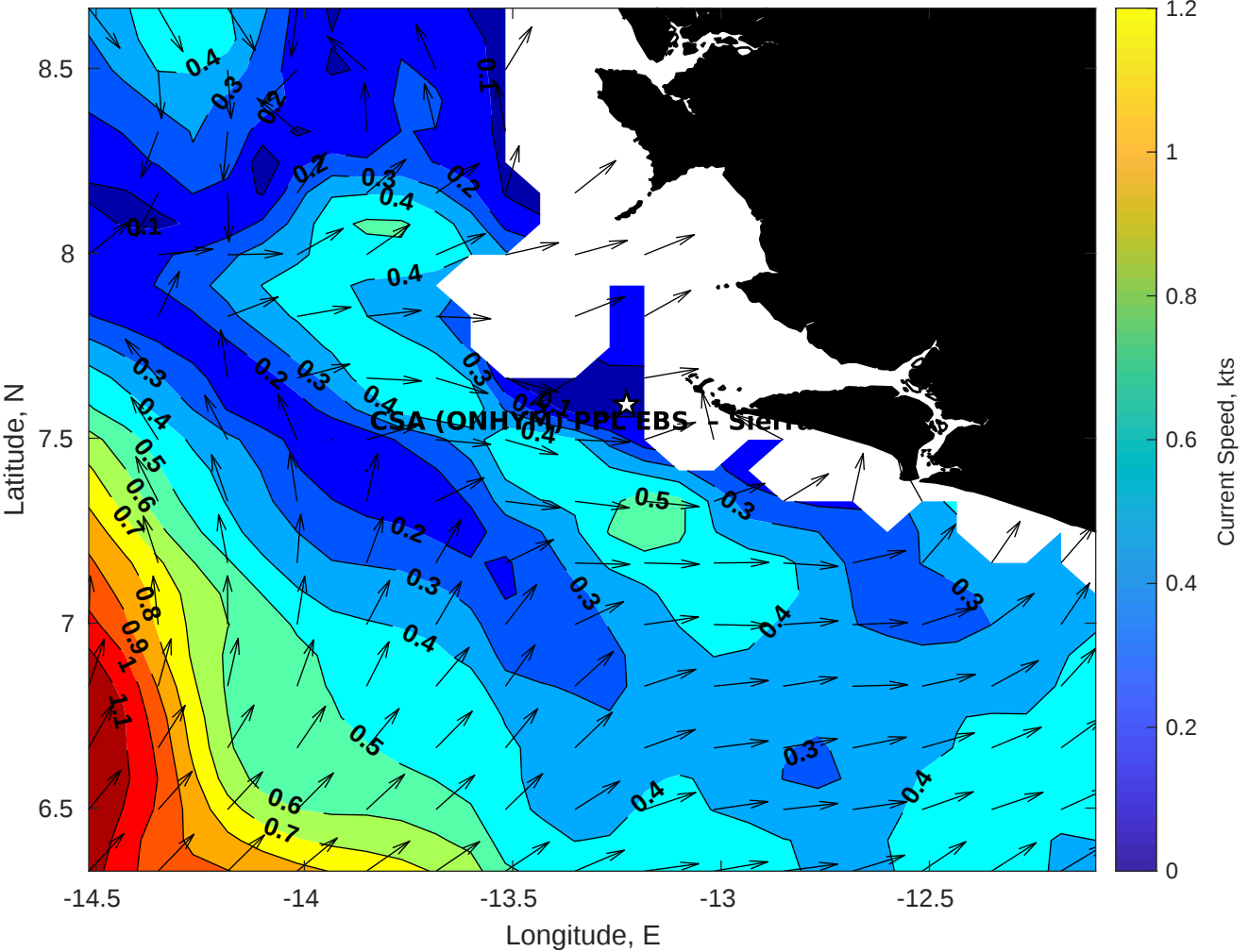
Surface Currents for CSA (ONHYM) PPL EBS - Sierra Leone at 30-Apr-2025 00:00:00
