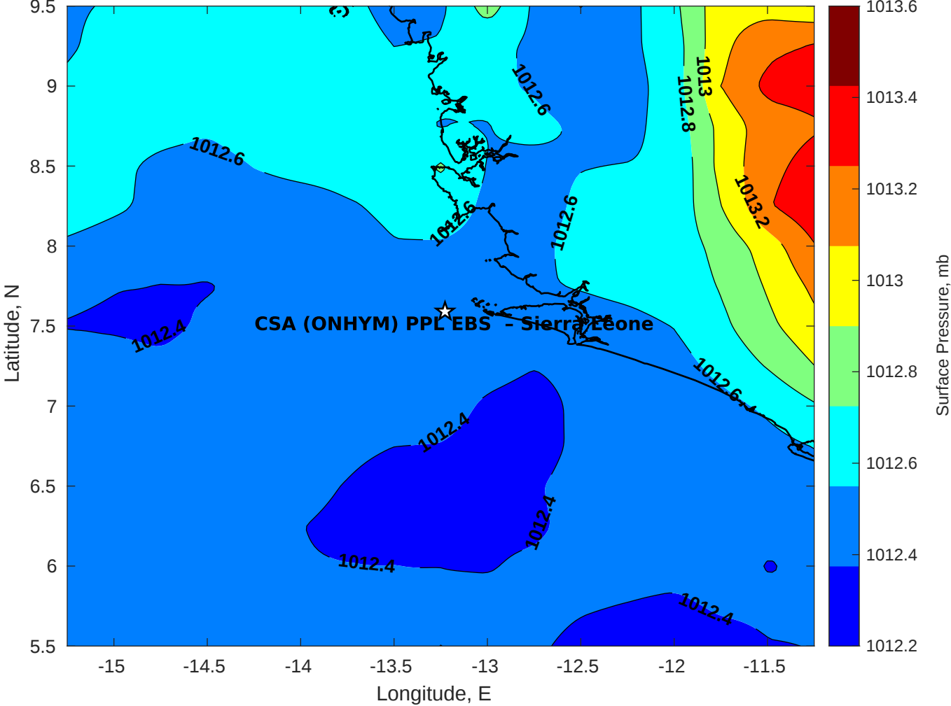
Surface Pressure (mb) for CSA (ONHYM) PPL EBS - Sierra Leone at 02-May-2025 00:00:00
