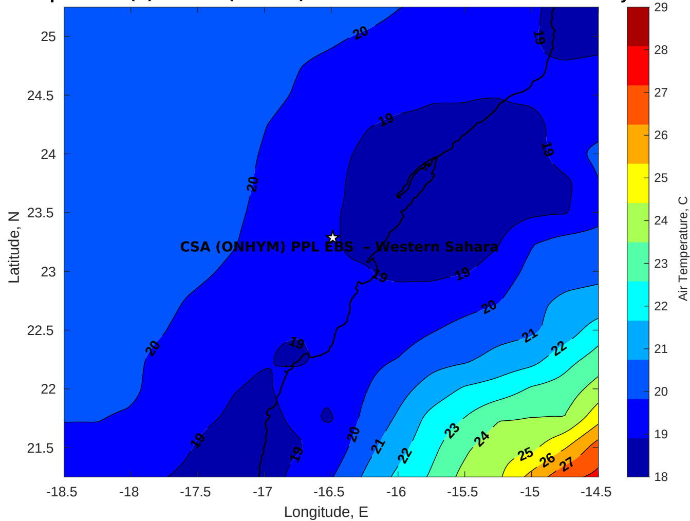
Air Temperature (C) for CSA (ONHYM) PPL EBS - Western Sahara at 01-May-2025
