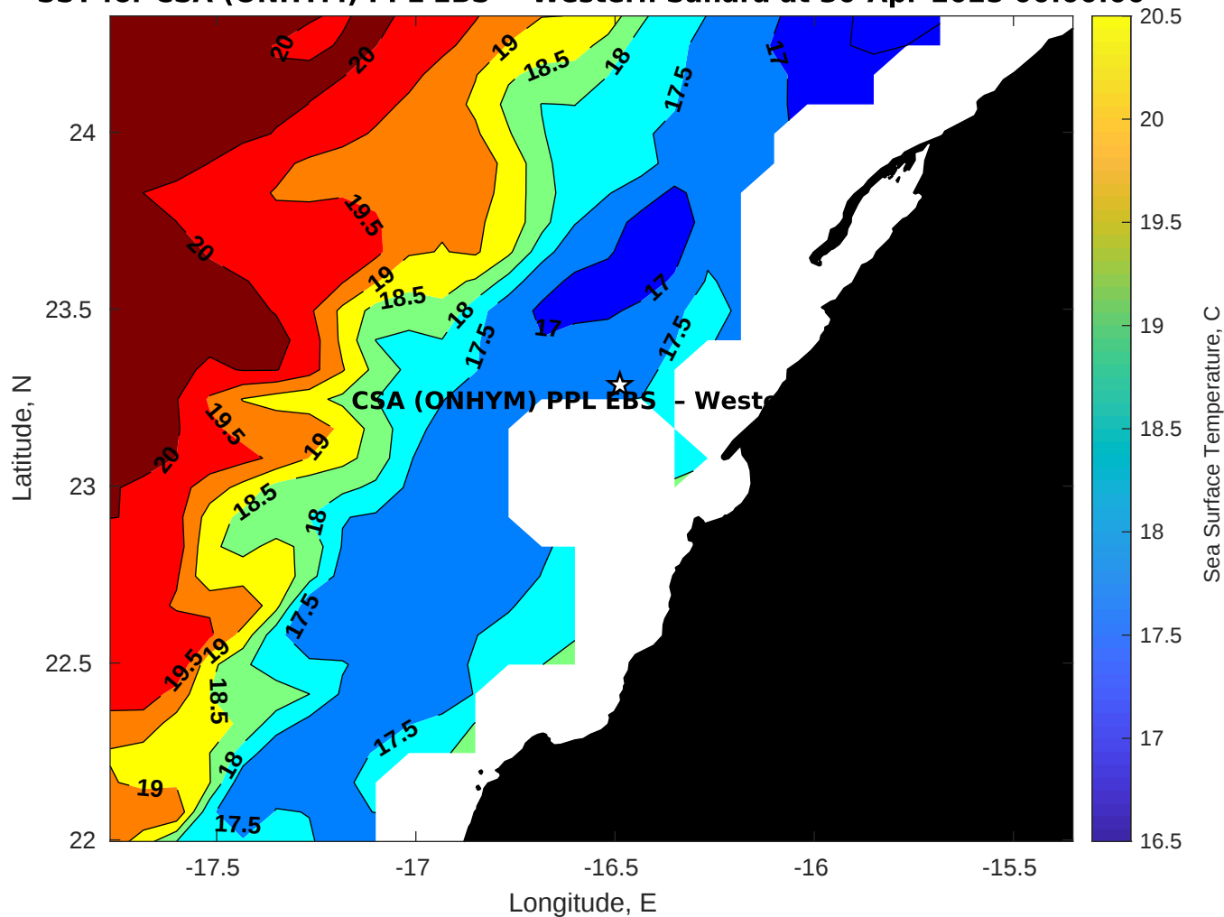
SST for CSA (ONHYM) PPL EBS - Western Sahara at 30-Apr-2025 00:00:00
