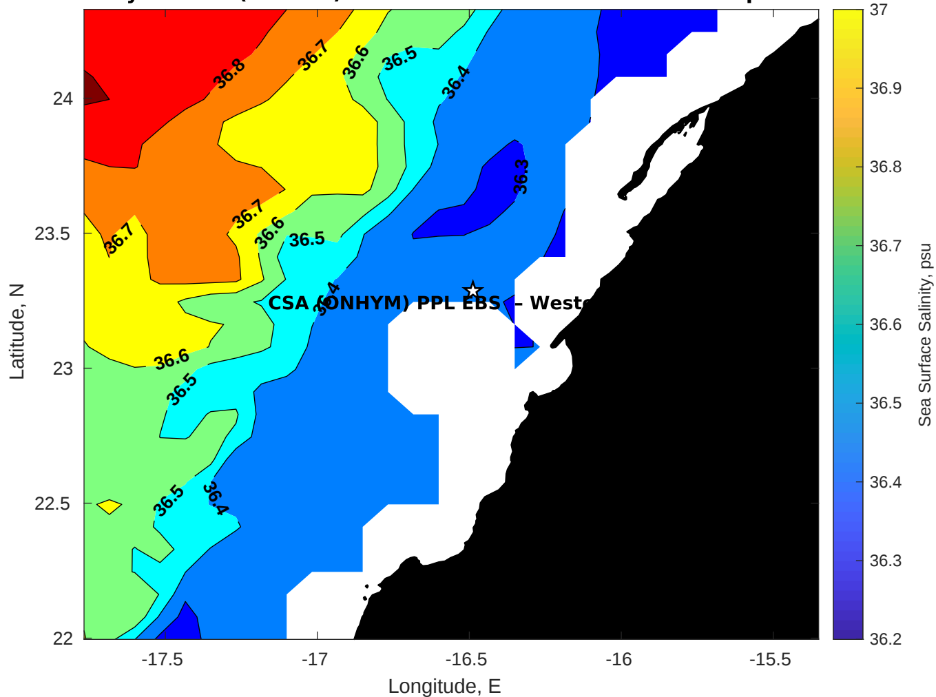
Surface Salinity for CSA (ONHYM) PPL EBS - Western Sahara at 30-Apr-2025 00:00:00
