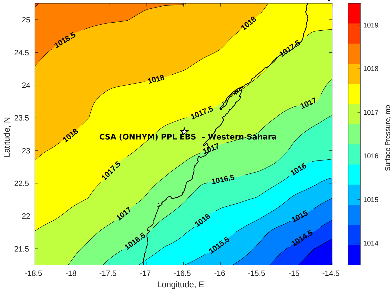
Surface Pressure (mb) for CSA (ONHYM) PPL EBS - Western Sahara at 03-May-2025 00:00:00
