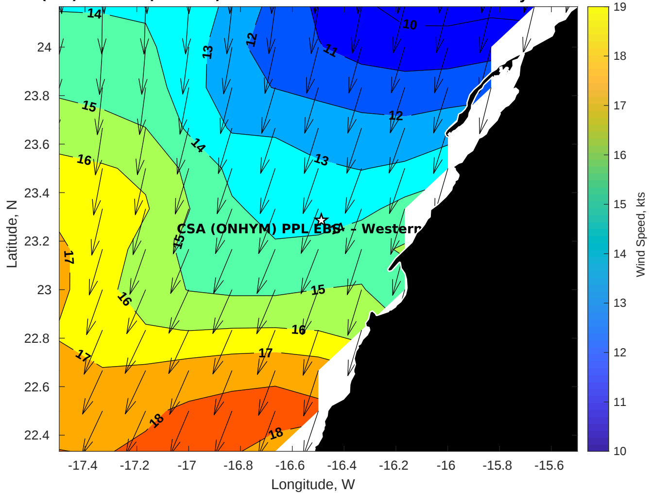
Winds (kts) for CSA (ONHYM) PPL EBS - Western Sahara at 01-May-2025 09:00:00
