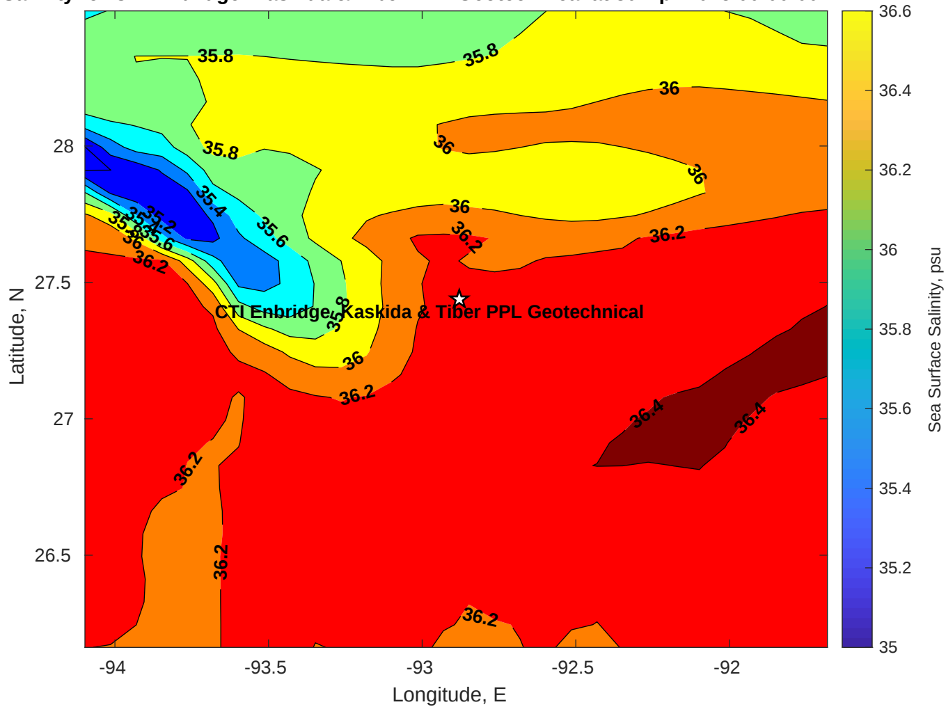
Surface Salinity for CTI Enbridge Kaskida & Tiber PPL Geotechnical at 30-Apr-2025 00:00:00
