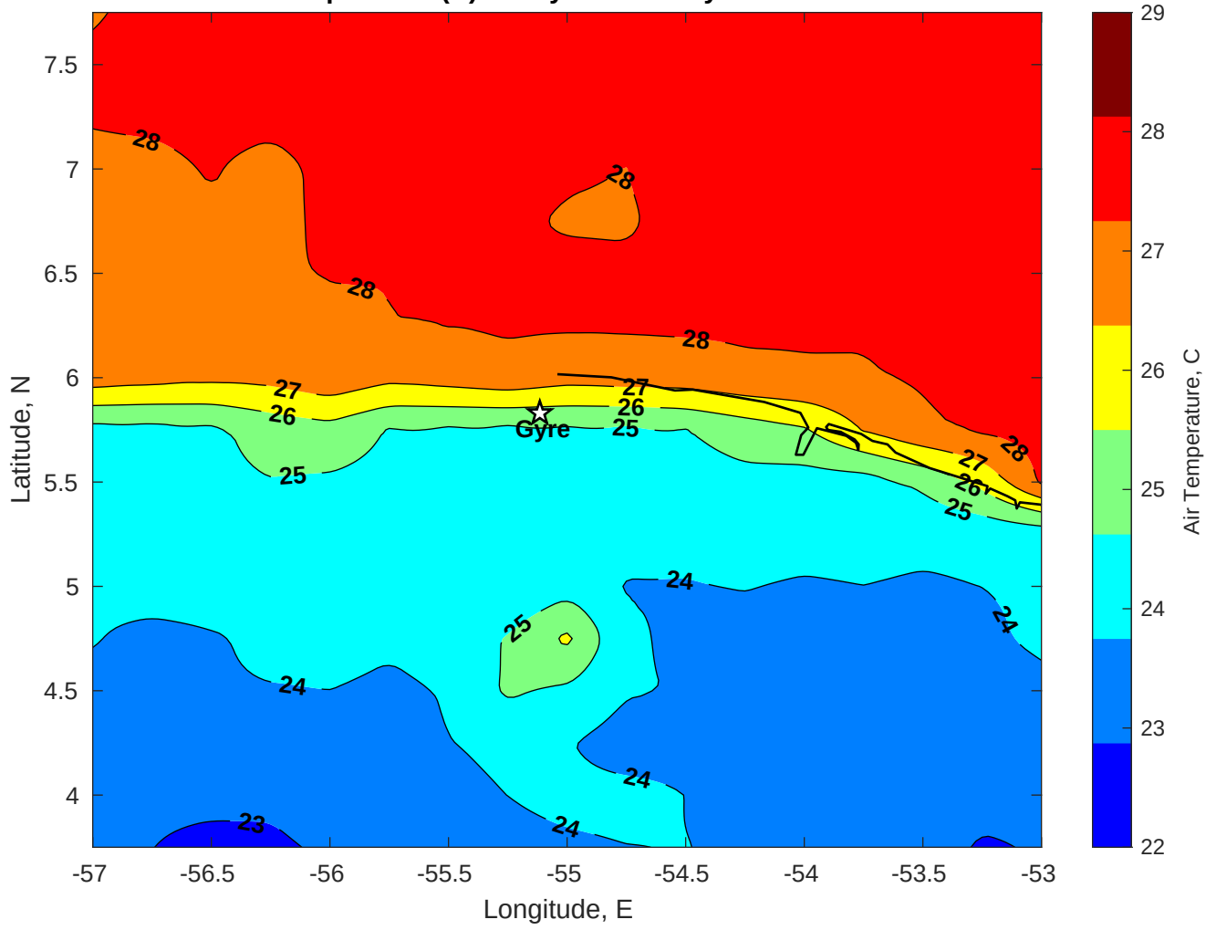
Air Temperature (C) for Gyre at 01-May-2025
