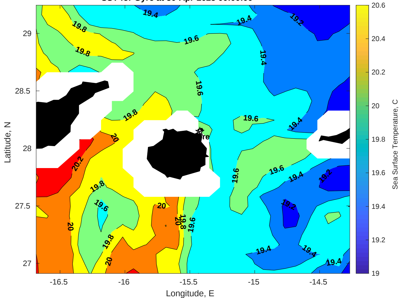
SST for Gyre at 30-Apr-2025 00:00:00
