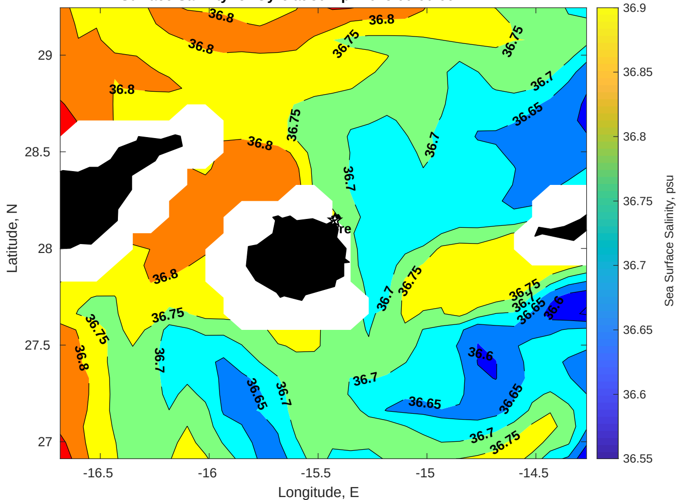
Surface Salinity for Gyre at 30-Apr-2025 00:00:00
