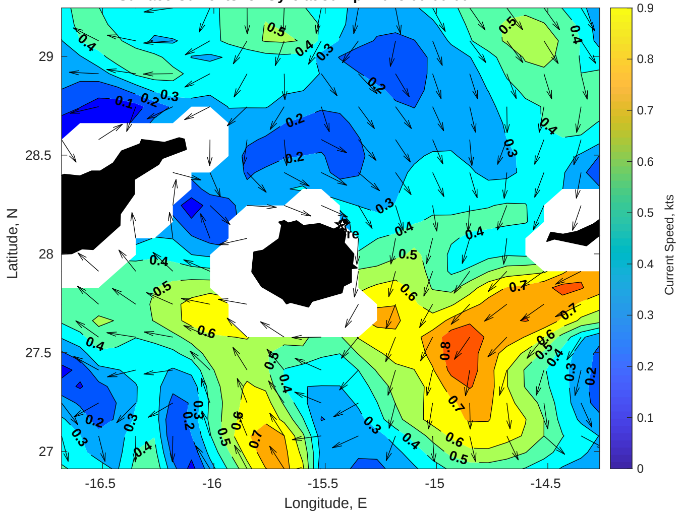
Surface Currents for Gyre at 30-Apr-2025 00:00:00
