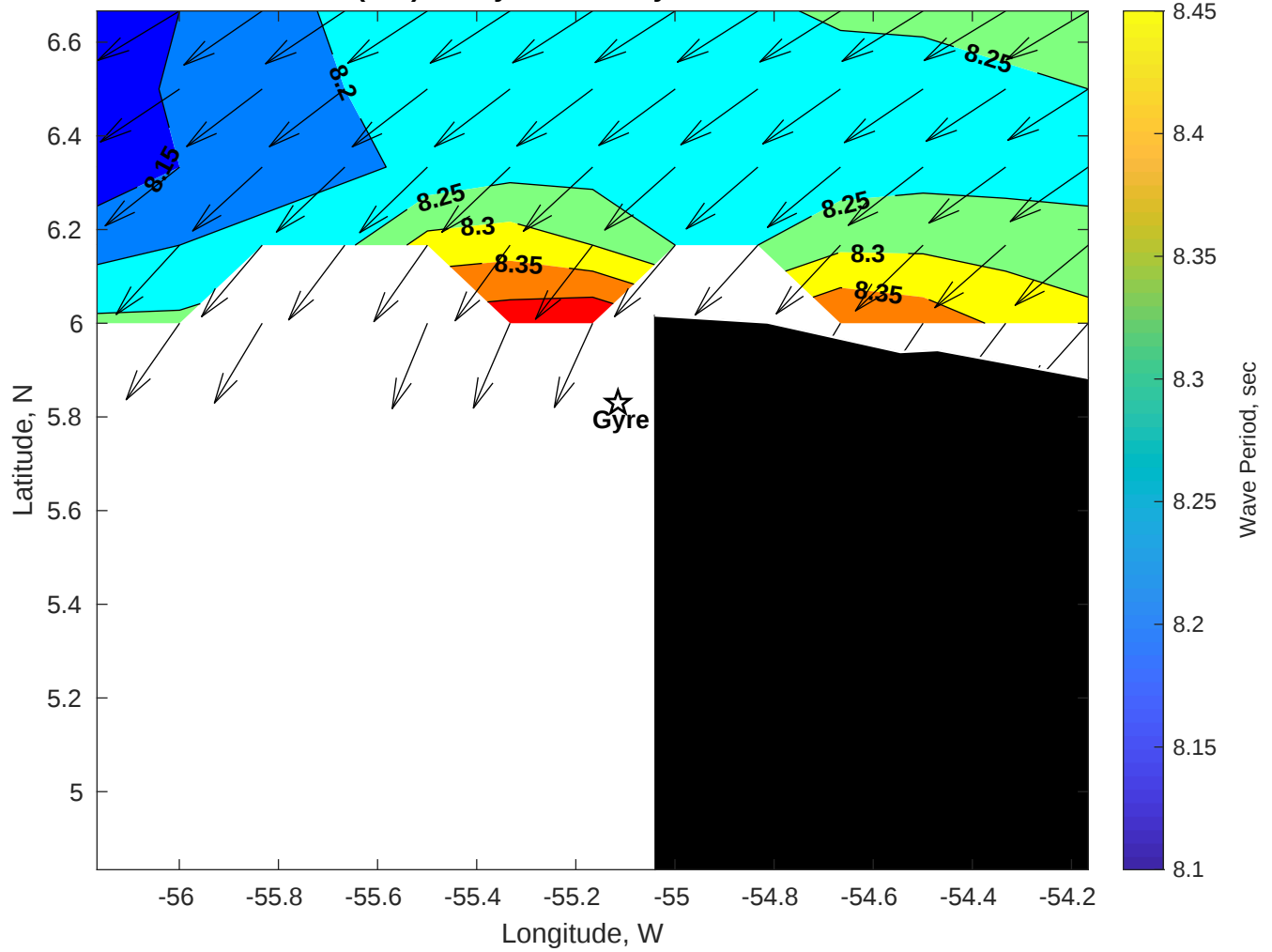
Wave Period (sec) for Gyre at 01-May-2025 09:00:00
