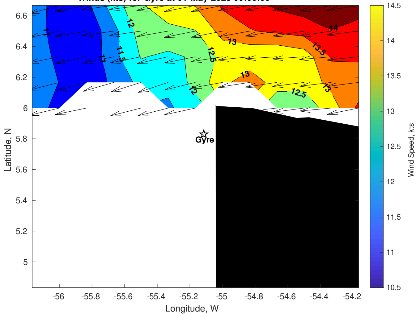
Winds (kts) for Gyre at 01-May-2025 09:00:00
