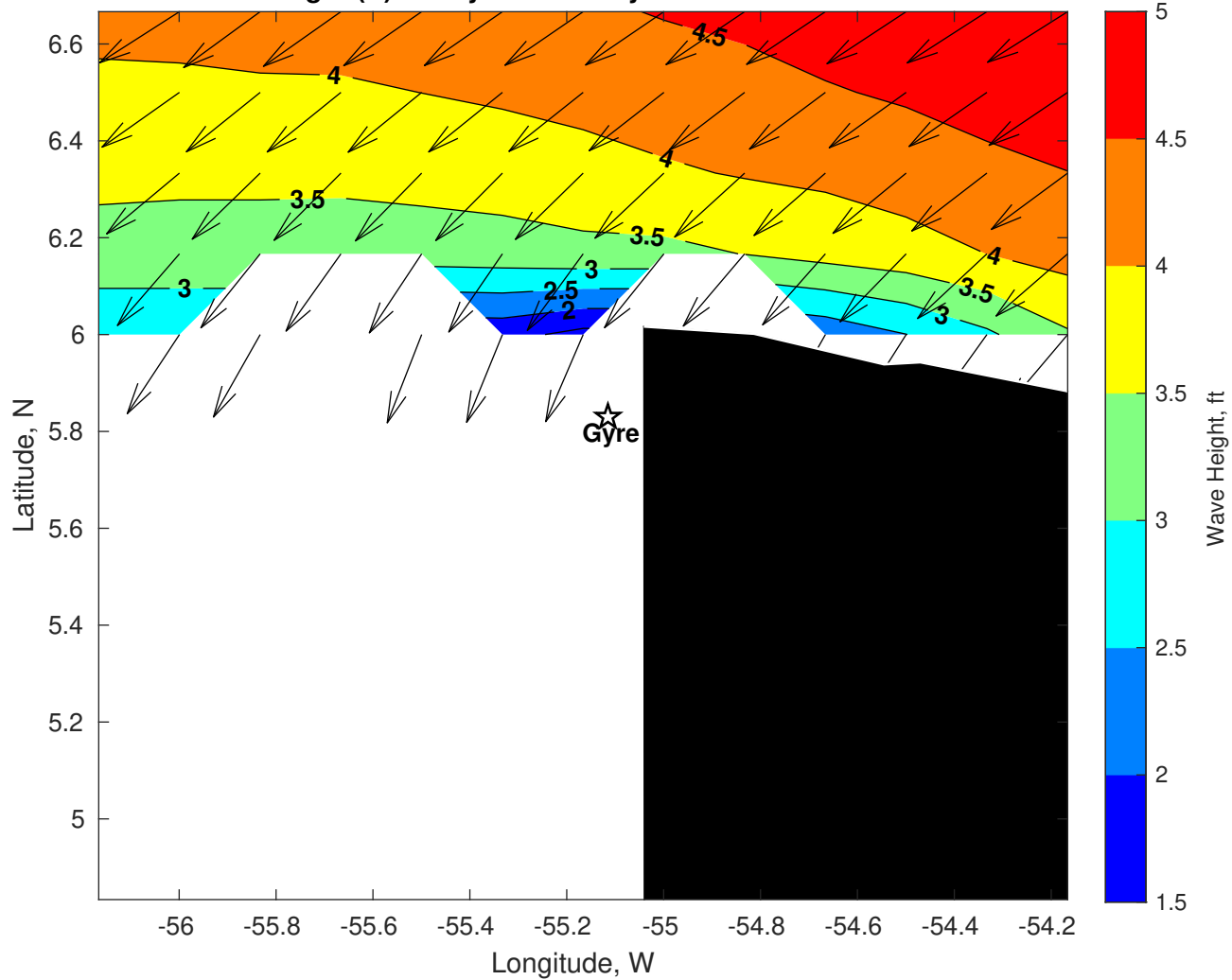
Wave Height (ft) for Gyre at 01-May-2025 09:00:00
