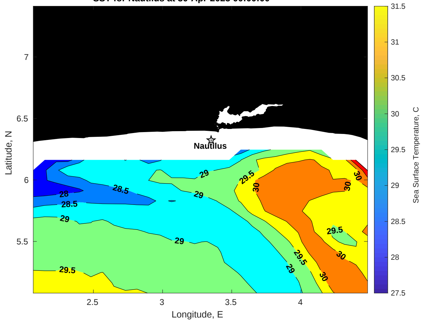
SST for Nautilus at 30-Apr-2025 00:00:00
