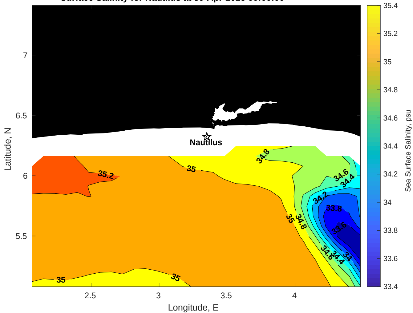
Surface Salinity for Nautilus at 30-Apr-2025 00:00:00
