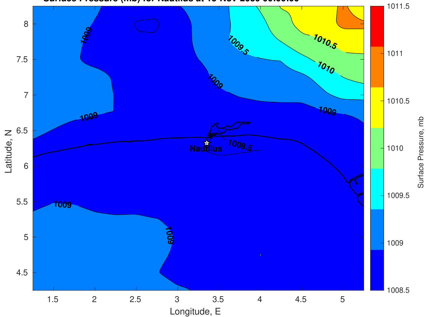
Surface Pressure (mb) for Nautilus at 15-Nov-2030 00:00:00
