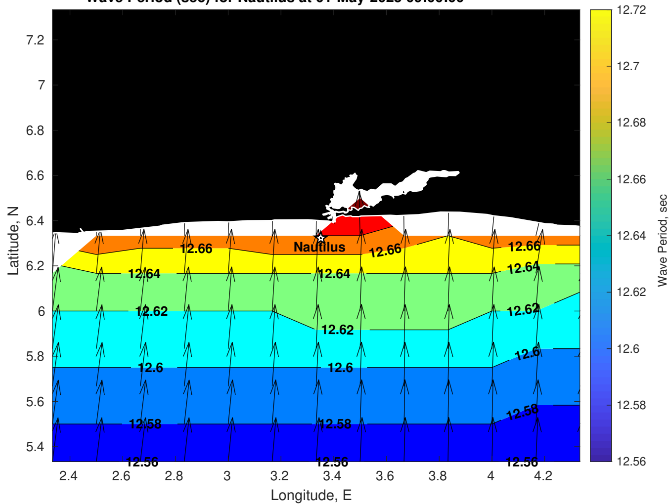
Wave Period (sec) for Nautilus at 01-May-2025 09:00:00
