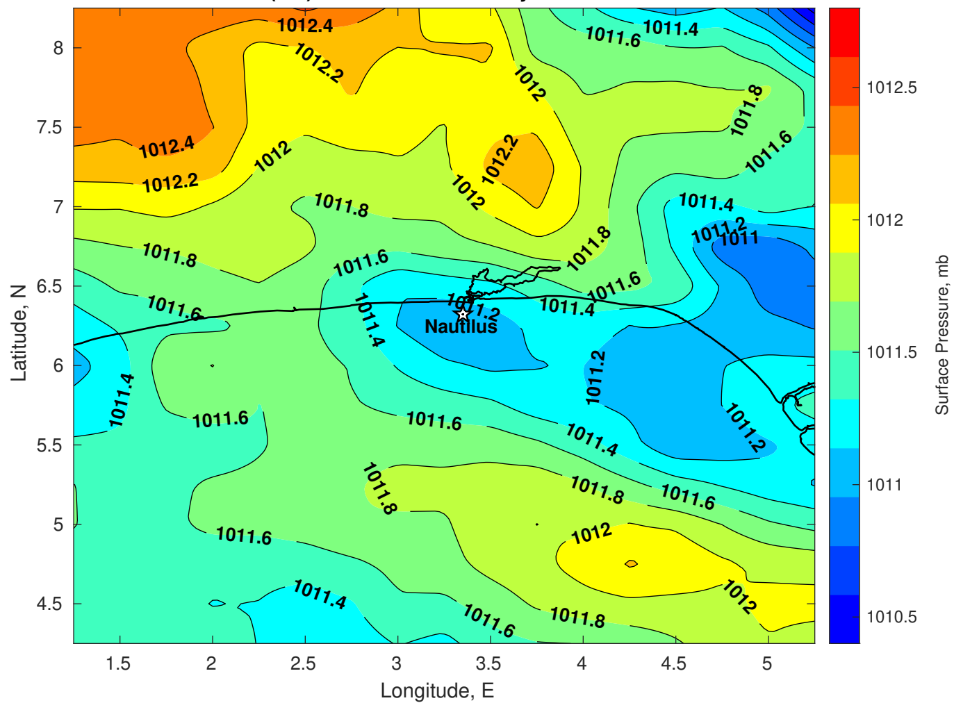
Surface Pressure (mb) for Nautilus at 03-May-2025 00:00:00
