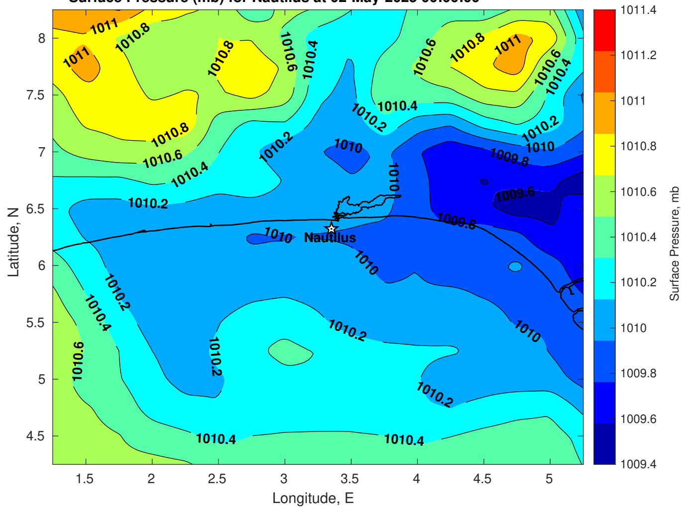
Surface Pressure (mb) for Nautilus at 02-May-2025 00:00:00
