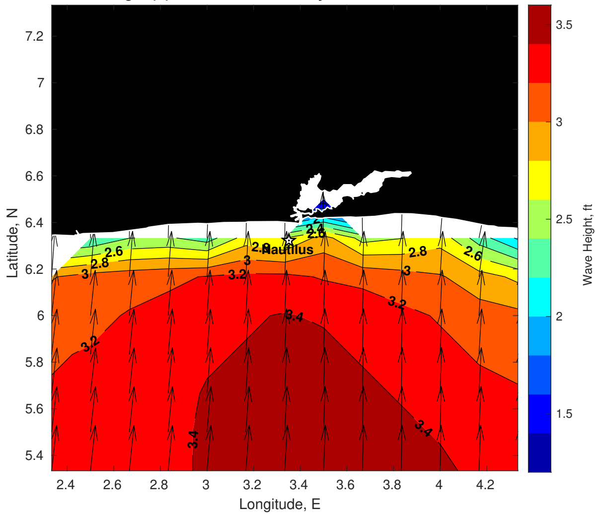
Wave Height (ft) for Nautilus at 01-May-2025 09:00:00
