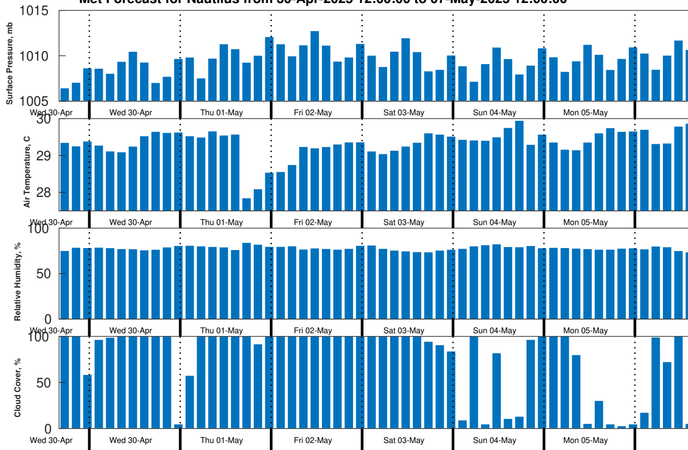
Met Forecast for Nautilus from 30-Apr-2025 12:00:00 to 07-May-2025 12:00:00
