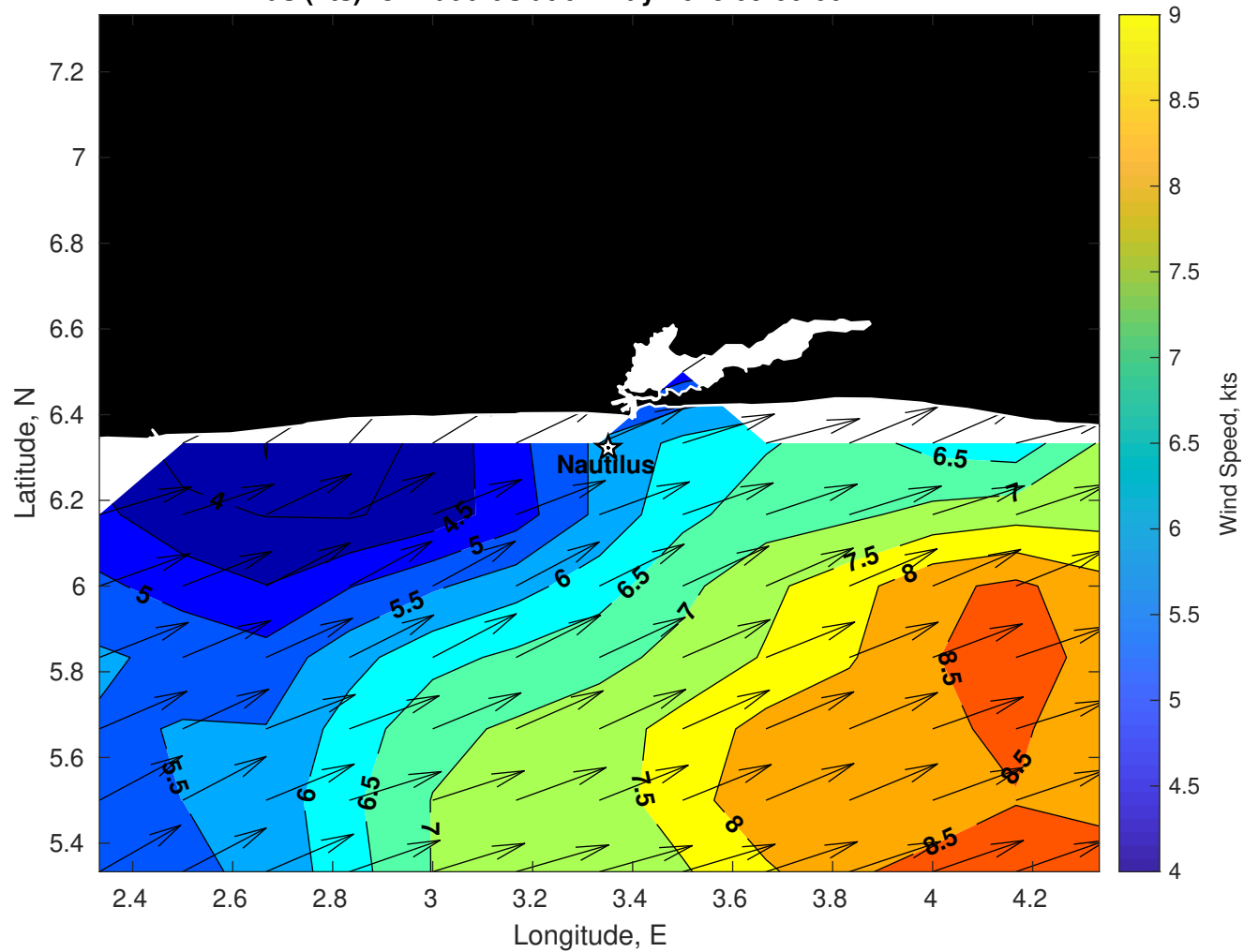
Winds (kts) for Nautilus at 01-May-2025 09:00:00
