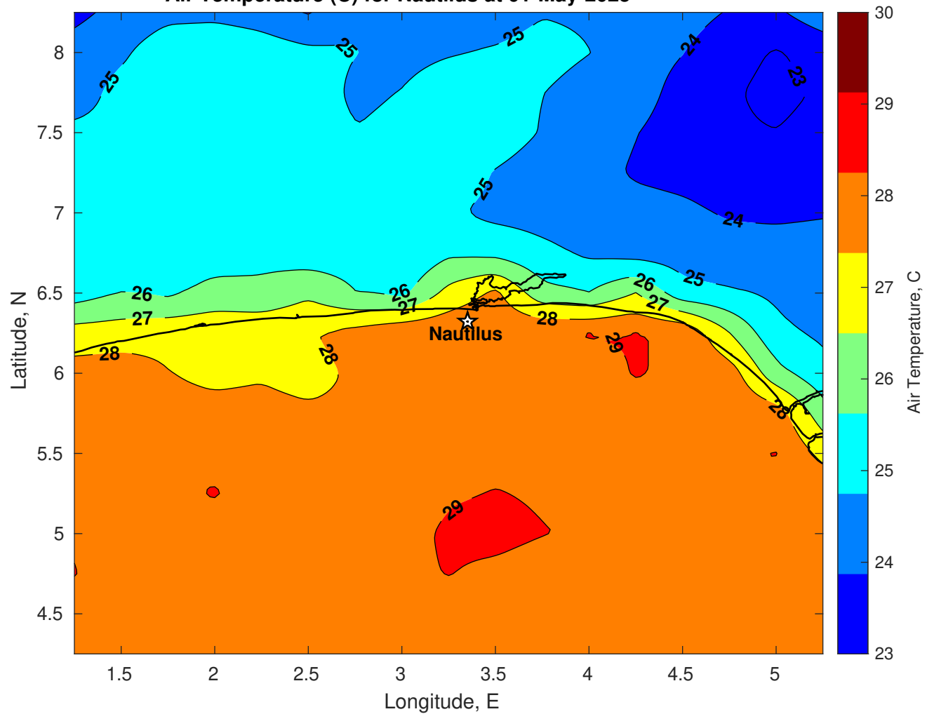
Air Temperature (C) for Nautilus at 01-May-2025
