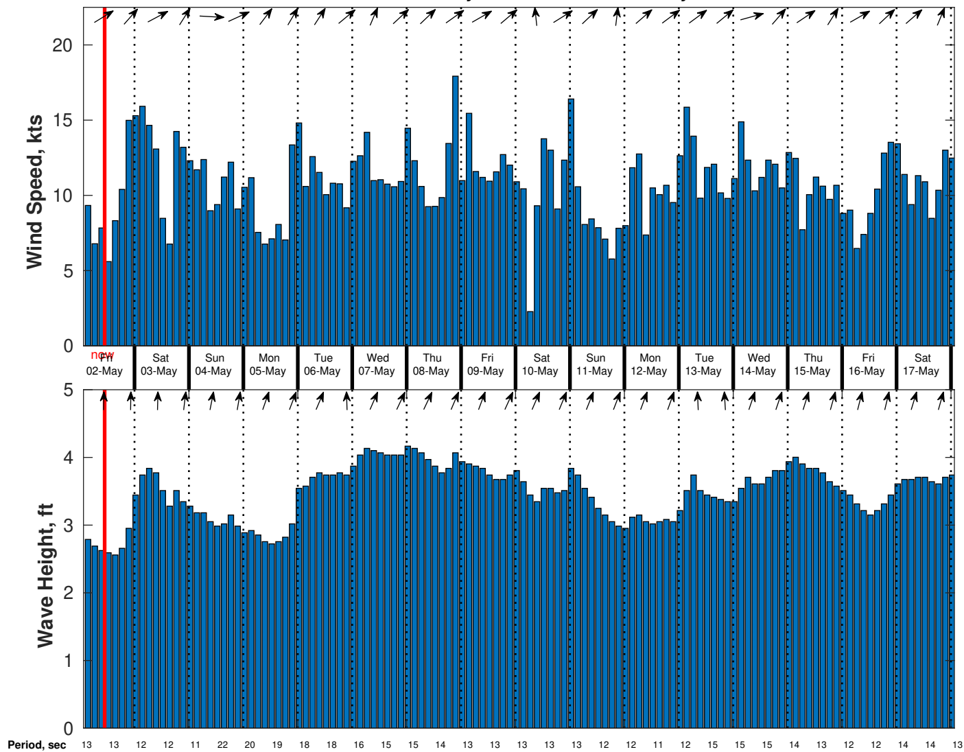
Wind & Wave Forecast for Nautilus from 01-May-2025 02:00:00 to 17-May-2025 02:00:00
