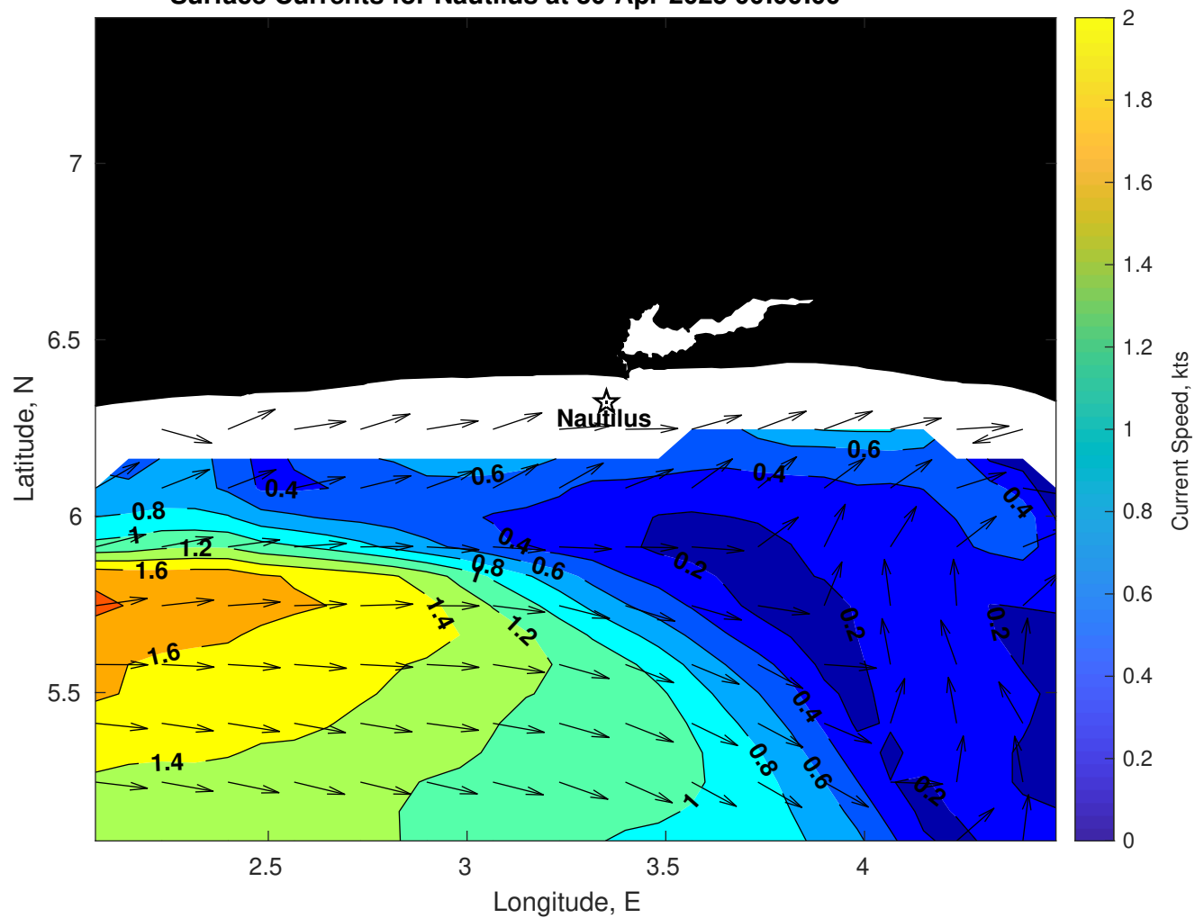
Surface Currents for Nautilus at 30-Apr-2025 00:00:00
