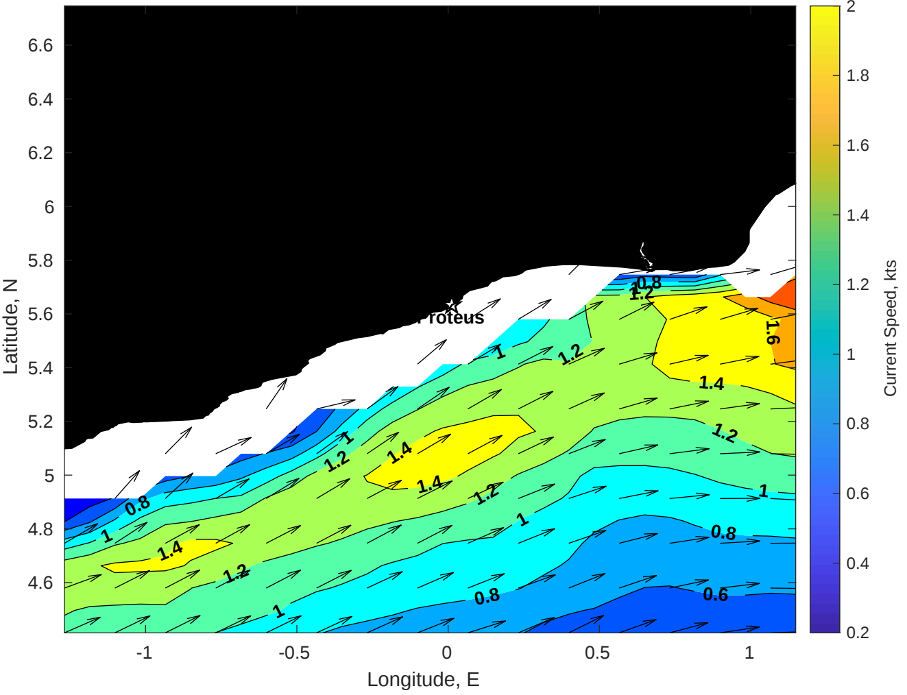
Surface Currents for Proteus at 30-Apr-2025 00:00:00
