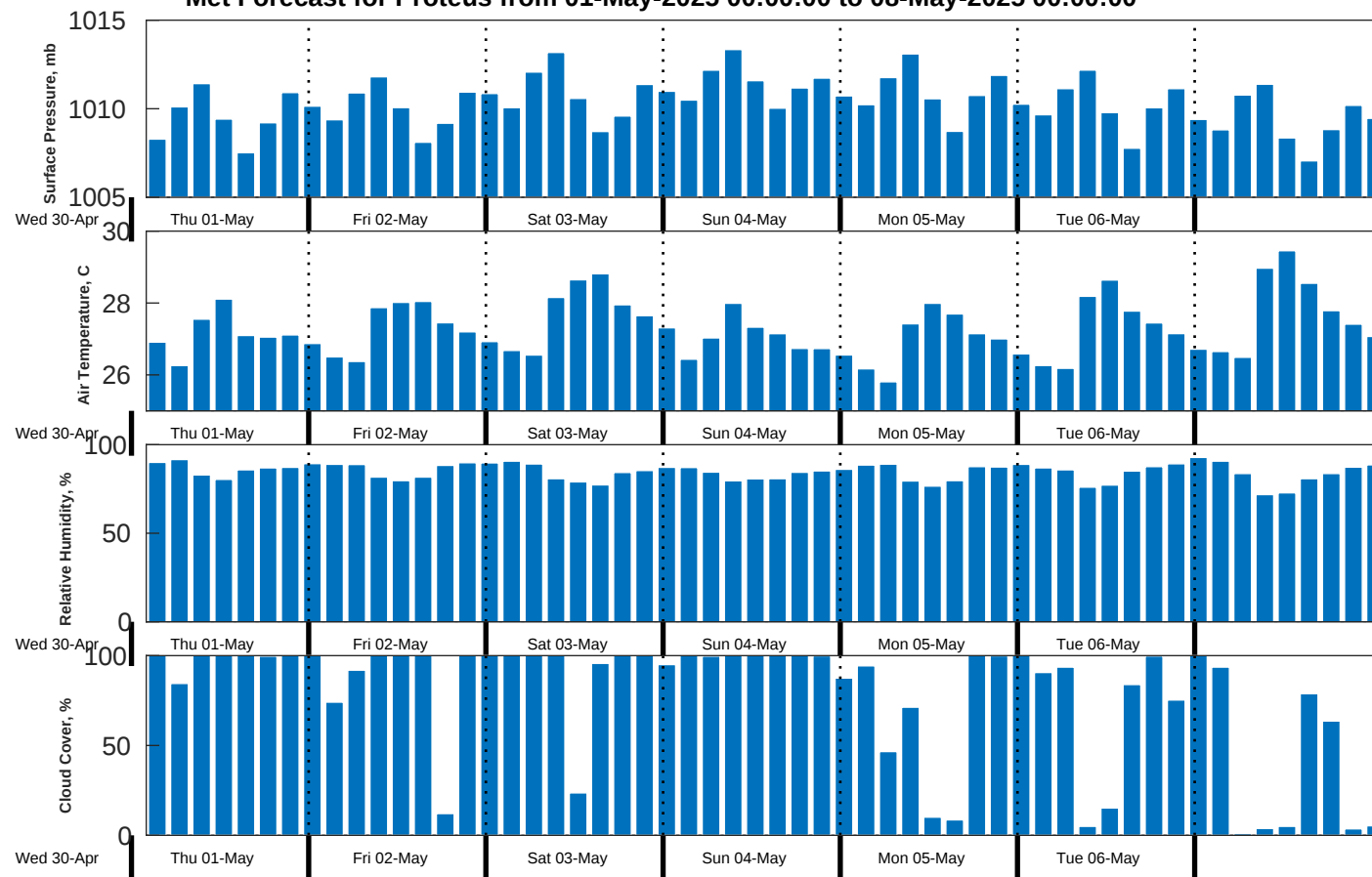
Met Forecast for Proteus from 01-May-2025 00:00:00 to 08-May-2025 00:00:00
