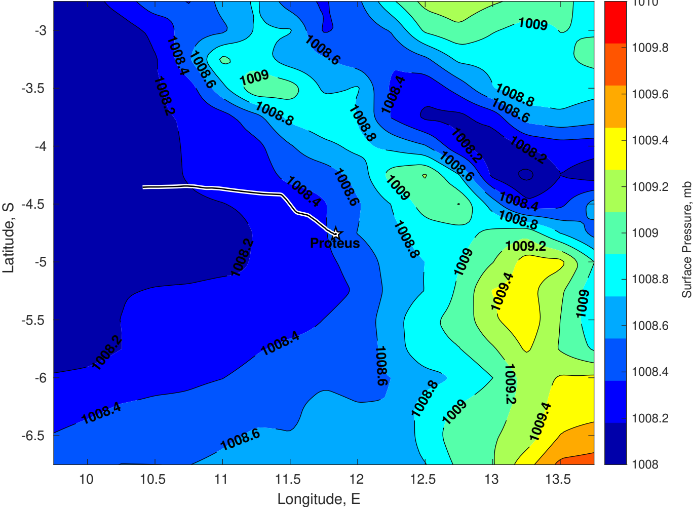
Surface Pressure (mb) for Proteus at 01-May-2025 00:00:00
