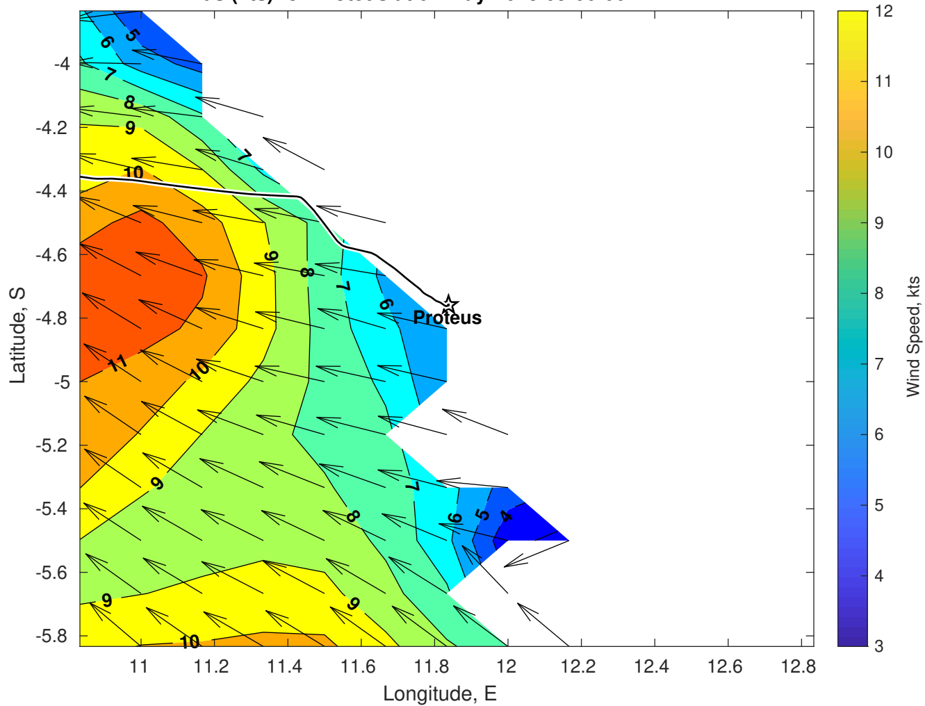
Winds (kts) for Proteus at 01-May-2025 09:00:00
