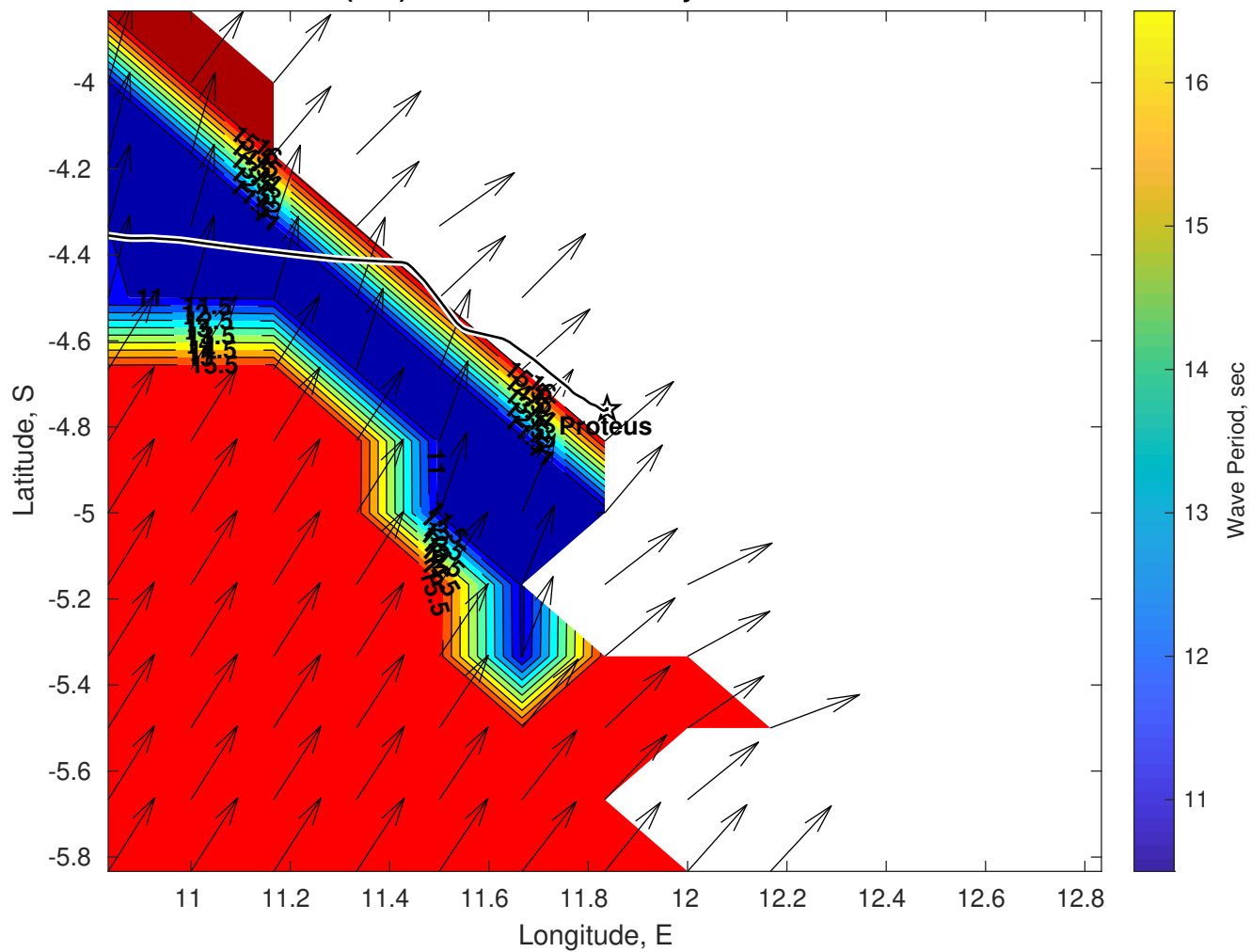
Wave Period (sec) for Proteus at 01-May-2025 09:00:00
