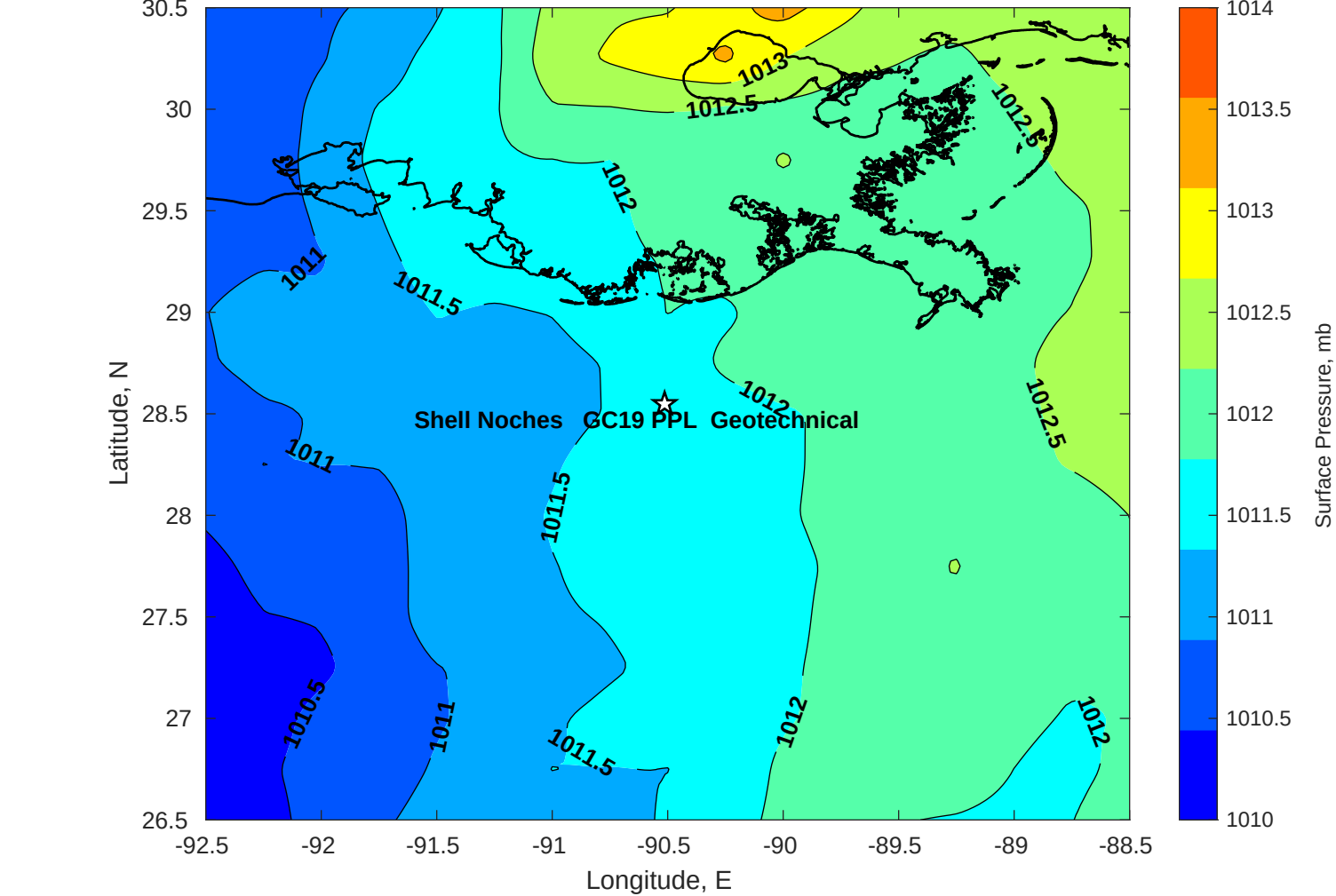
Surface Pressure (mb) for Shell Noches GC19 PPL Geotechnical at 03-May-2025 00:00:00
