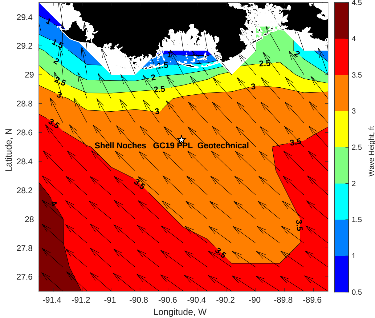
Wave Height (ft) for Shell Noches GC19 PPL Geotechnical at 01-May-2025 09:00:00
