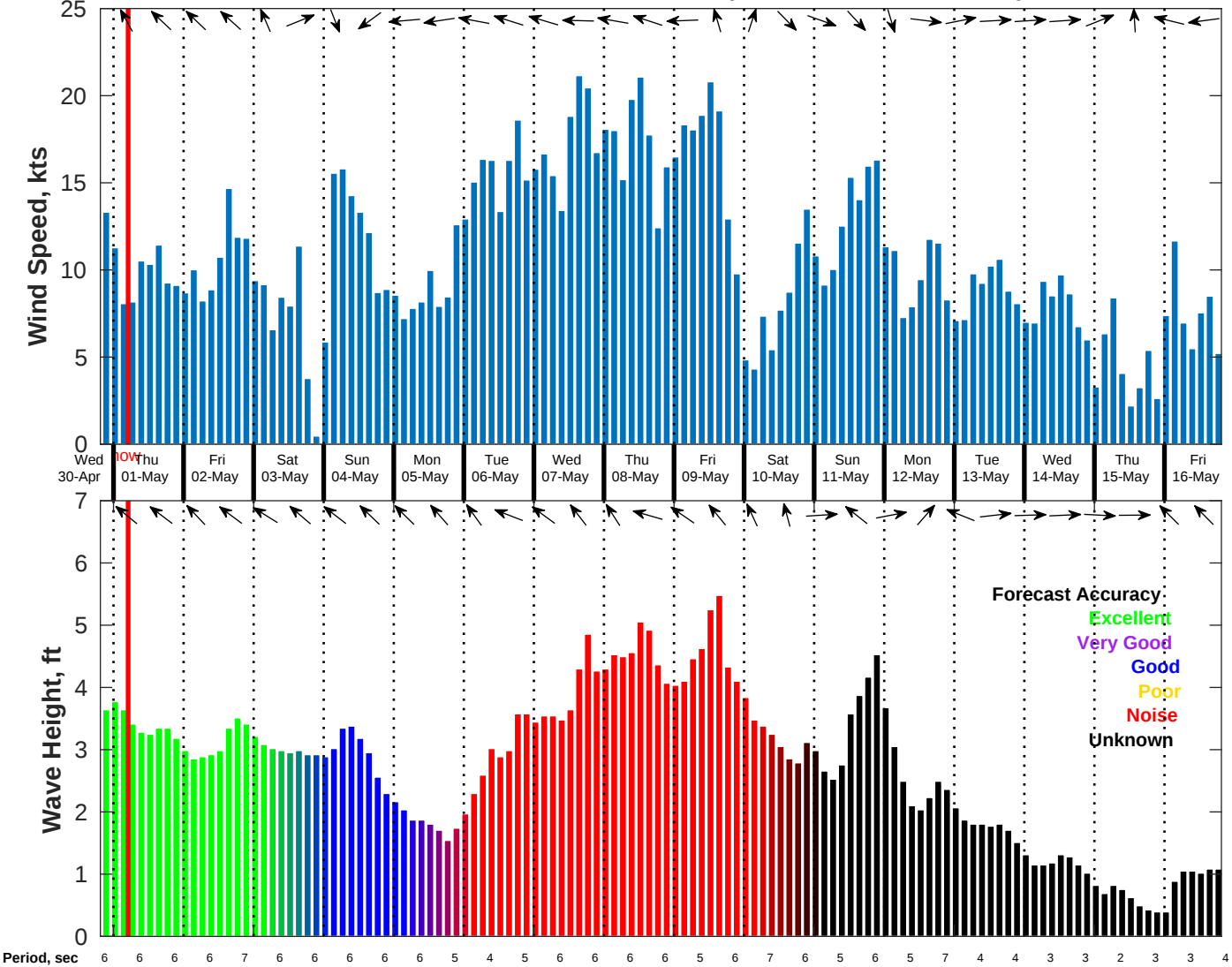
Wind & Wave Forecast for Shell Noches GC19 PPL Geotechnical from 30-Apr-2025 20:00:00 to 16-May-2025 20:00:00
