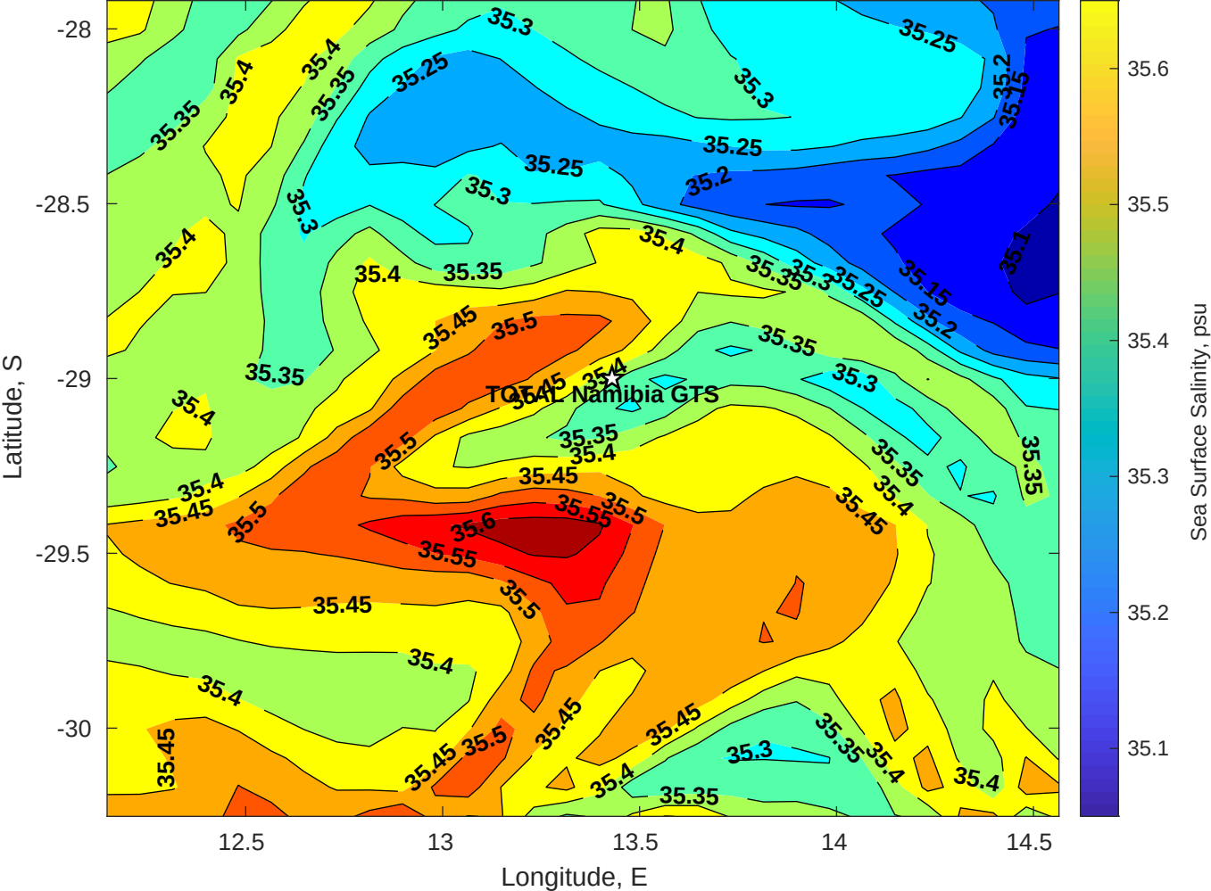
Surface Salinity for TOTAL Namibia GTS at 30-Apr-2025 00:00:00
