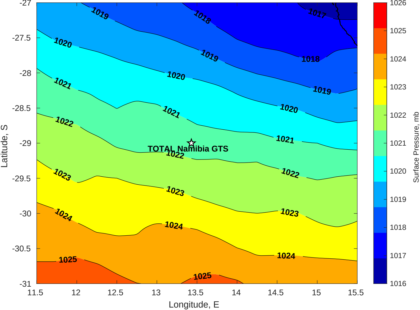
Surface Pressure (mb) for TOTAL Namibia GTS at 03-May-2025 00:00:00
