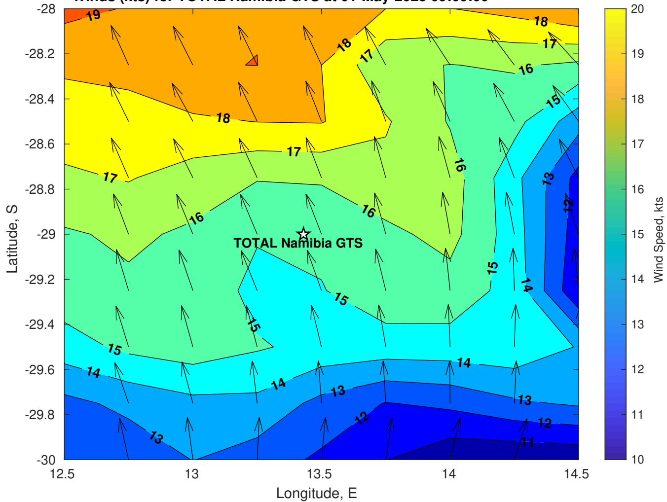
Winds (kts) for TOTAL Namibia GTS at 01-May-2025 09:00:00
