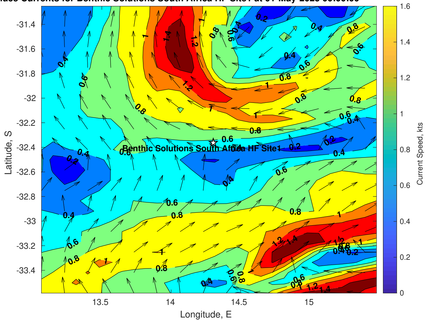
Surface Currents for Benthic Solutions South Africa HF Site1 at 01-May-2025 00:00:00
