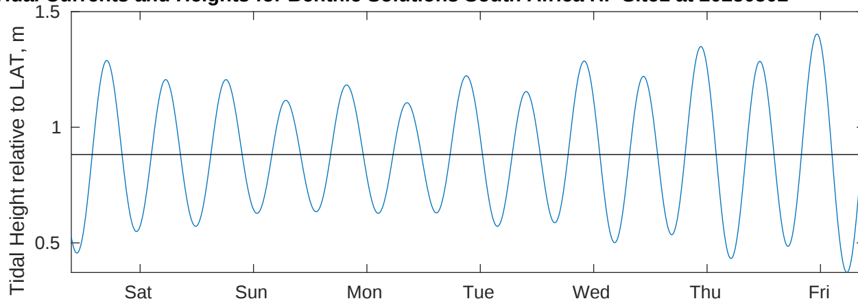
Tidal Currents and Heights for Benthic Solutions South Africa HF Site1 at 20250502
