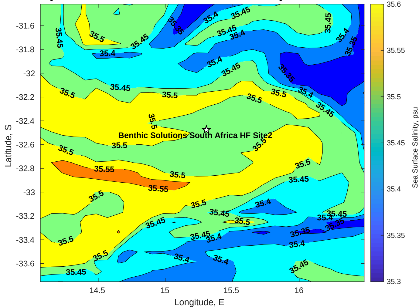
Surface Salinity for Benthic Solutions South Africa HF Site2 at 01-May-2025 00:00:00
