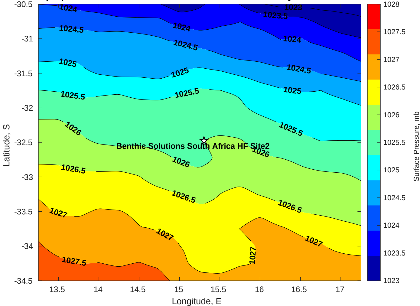
Surface Pressure (mb) for Benthic Solutions South Africa HF Site2 at 03-May-2025 00:00:00
