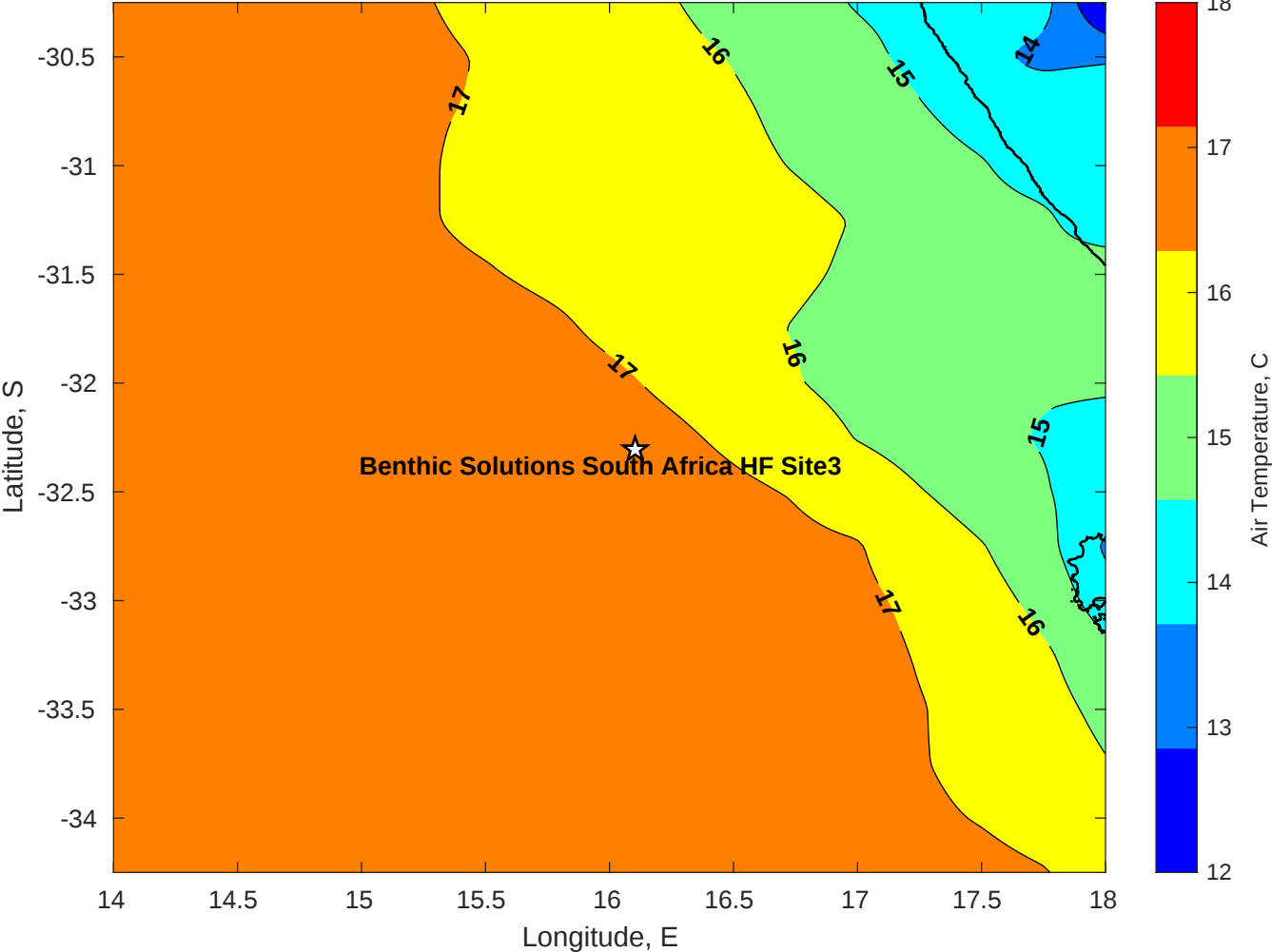
Air Temperature (C) for Benthic Solutions South Africa HF Site3 at 02-May-2025
