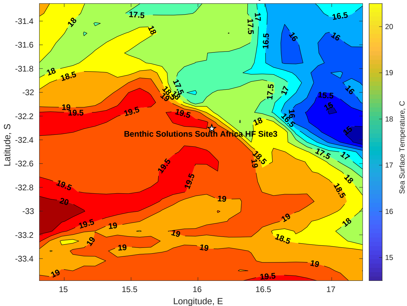
SST for Benthic Solutions South Africa HF Site3 at 01-May-2025 00:00:00
