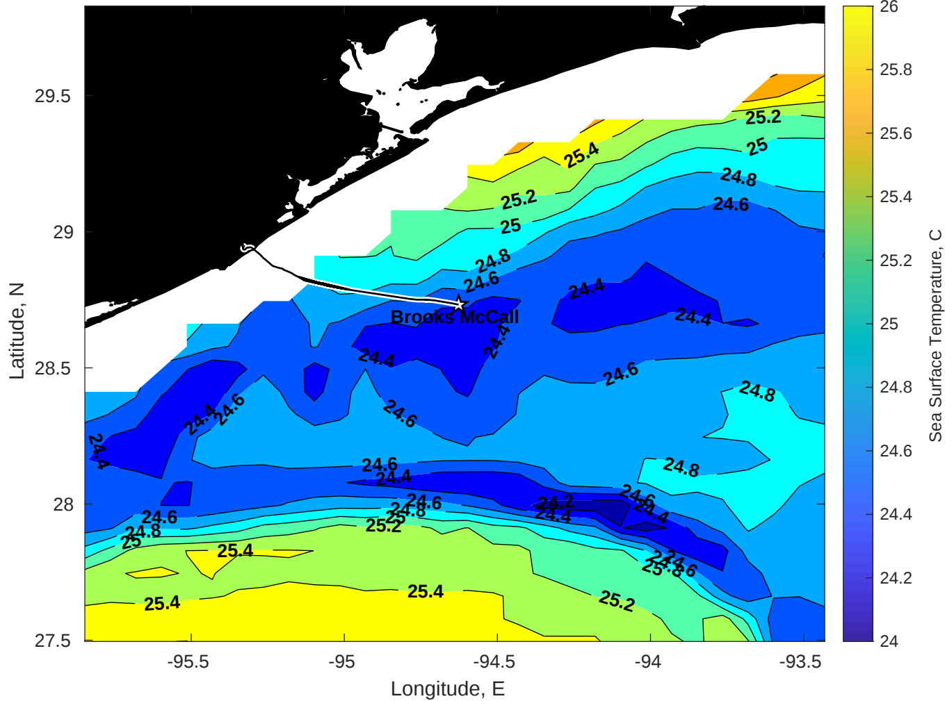
SST for Brooks McCall at 01-May-2025 00:00:00
