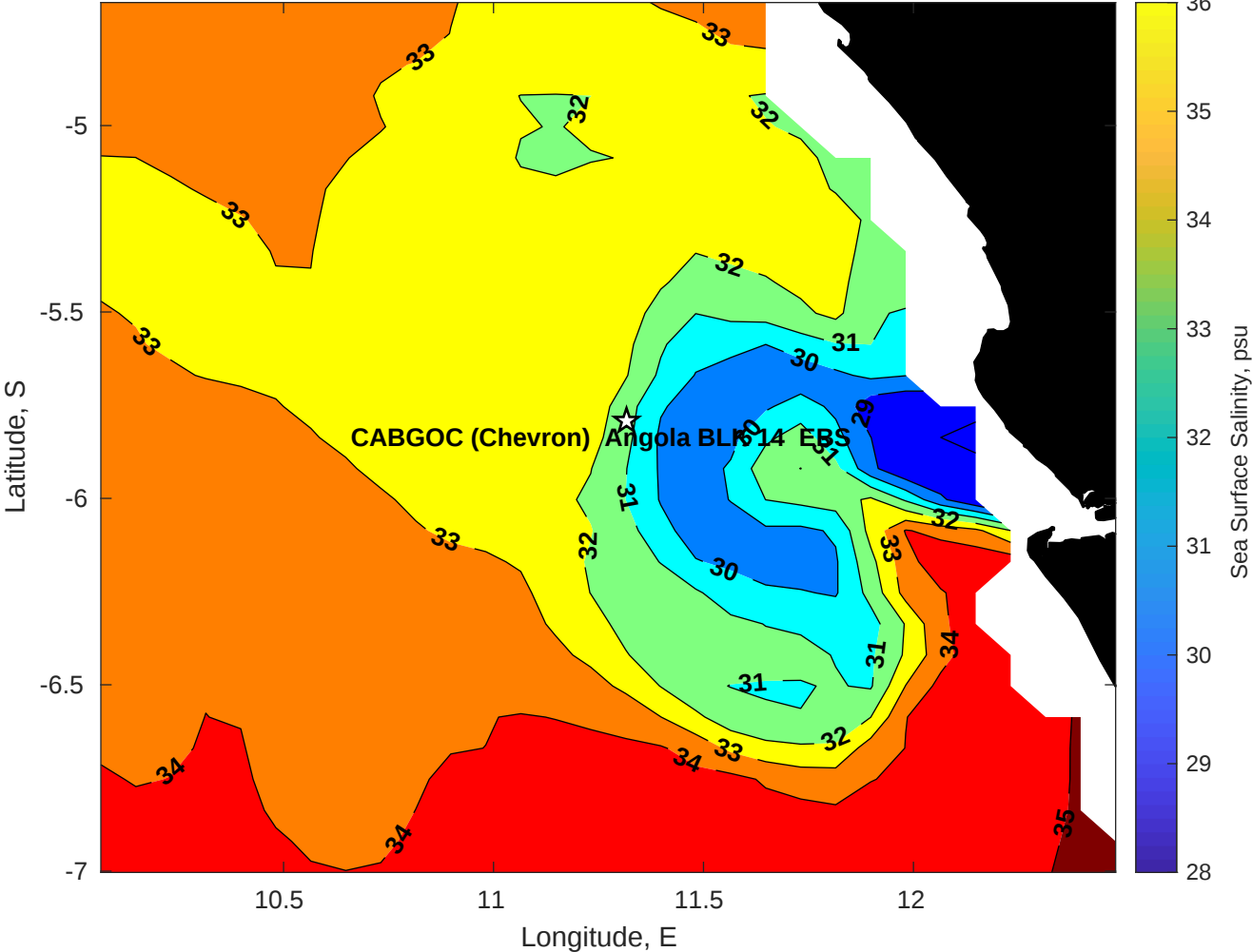
Surface Salinity for CABGOC (Chevron) Angola BLK 14 EBS at 01-May-2025 00:00:00
