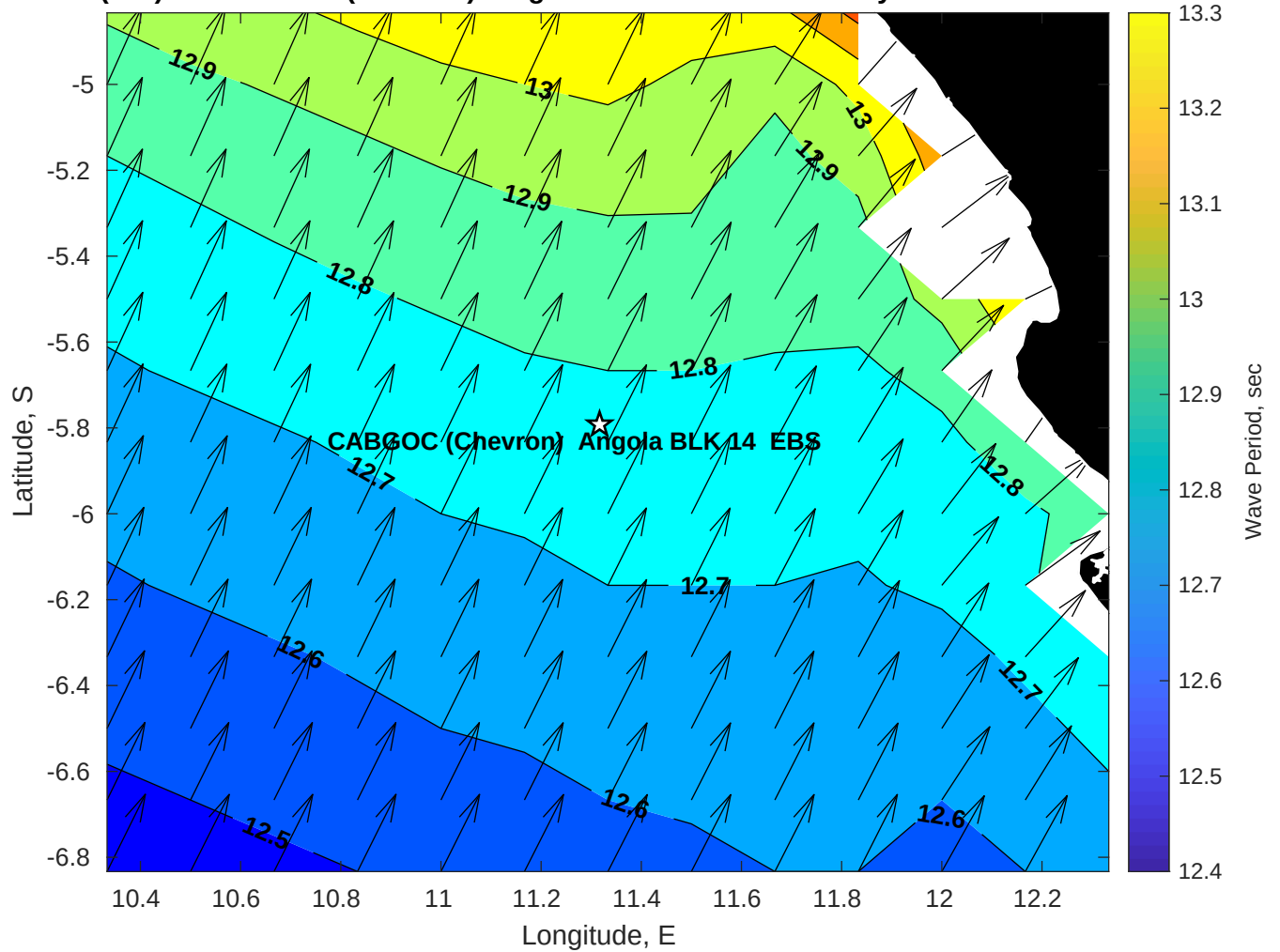
Wave Period (sec) for CABGOC (Chevron) Angola BLK 14 EBS at 02-May-2025 09:00:00
