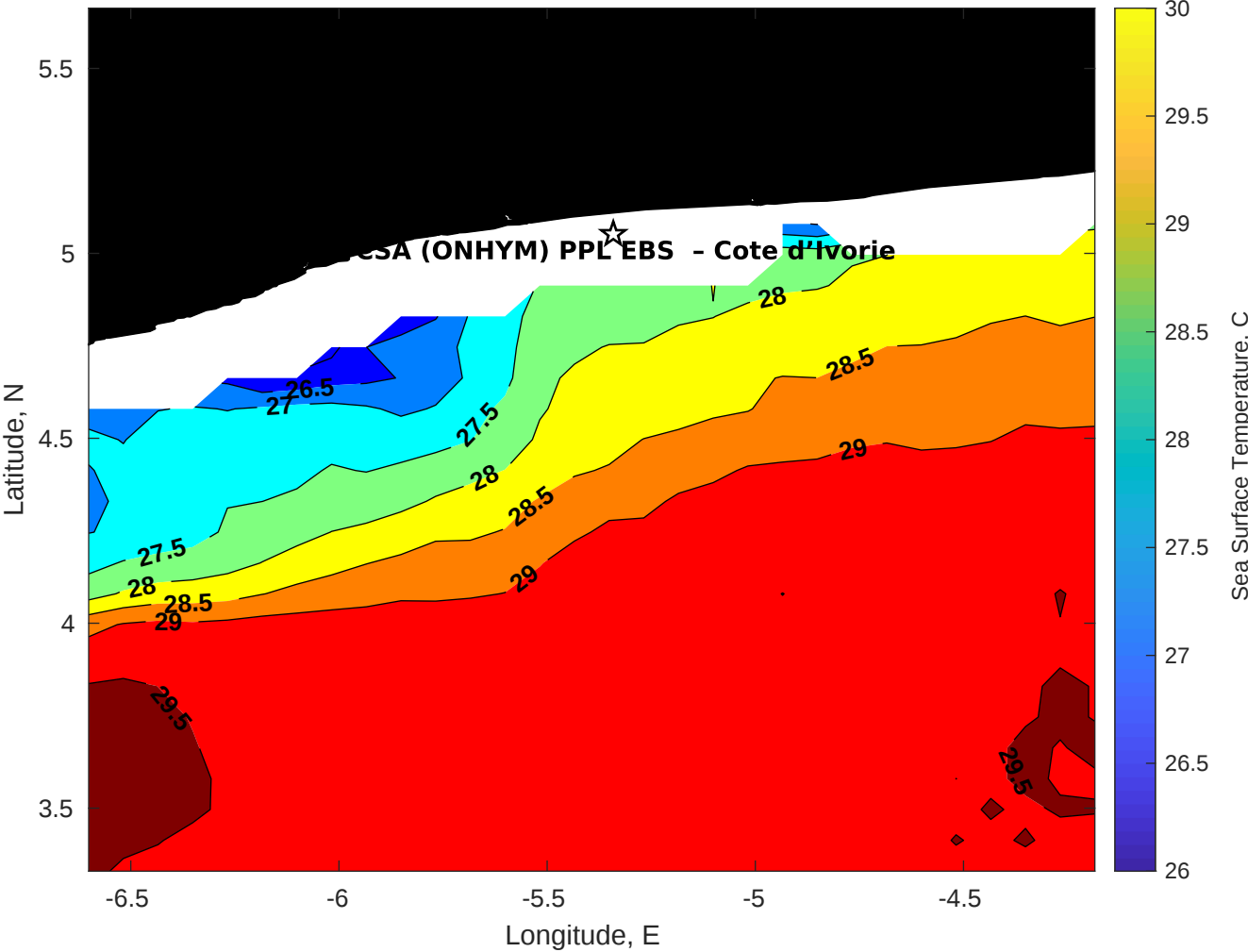
SST for CSA (ONHYM) PPL EBS - Cote d'Ivoire at 01-May-2025 00:00:00
