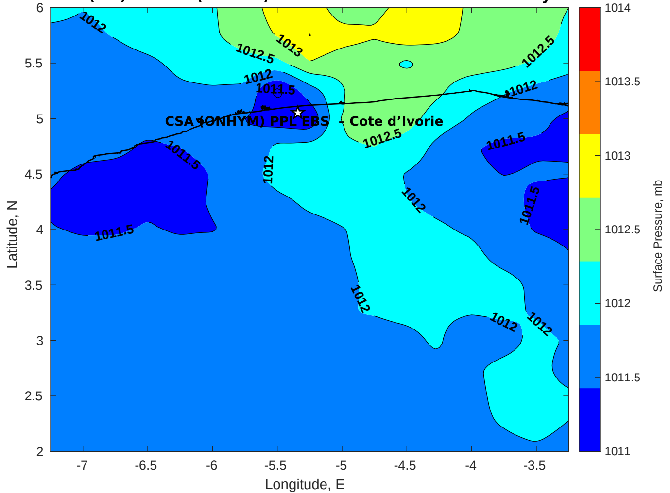
Surface Pressure (mb) for CSA (ONHYM) PPL EBS - Cote d'Ivoire at 02-May-2025 00:00:00
