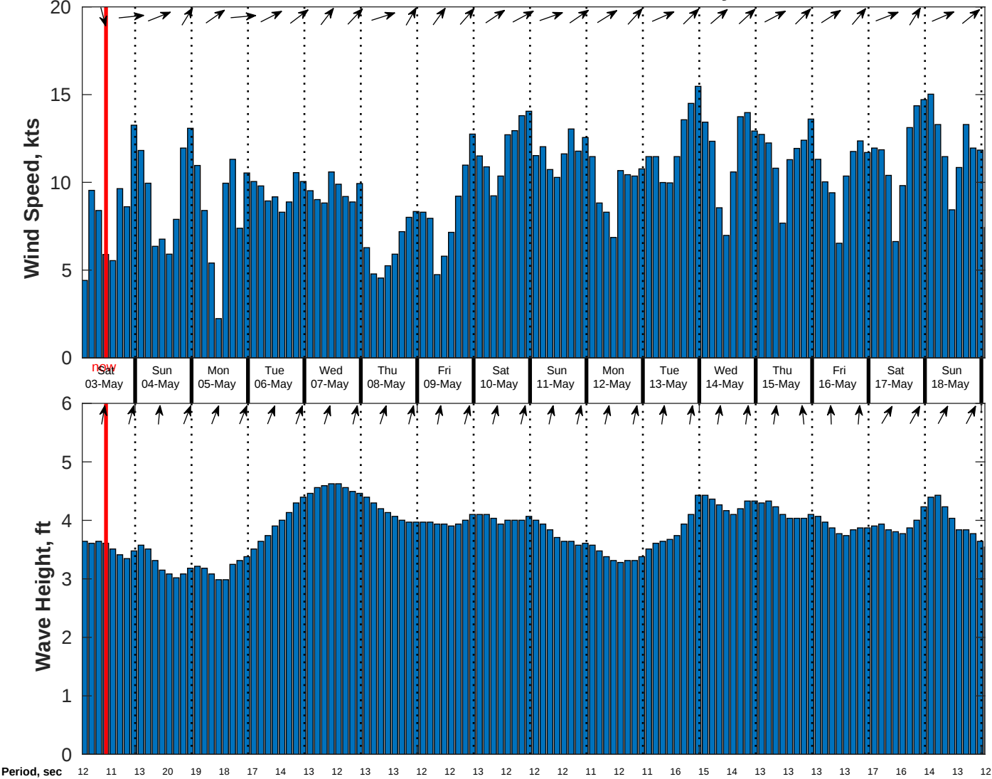
Wind & Wave Forecast for CSA (ONHYM) PPL EBS - Cote d'Ivoire from 02-May-2025 01:00:00 to 18-May-2025 01:00:00
