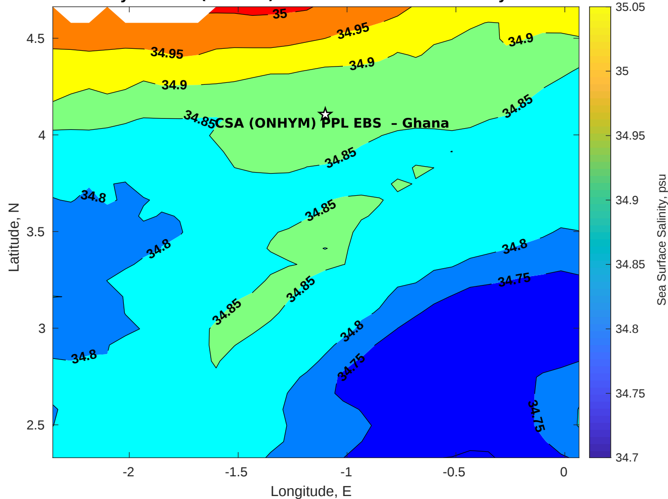
Surface Salinity for CSA (ONHYM) PPL EBS - Ghana at 01-May-2025 00:00:00
