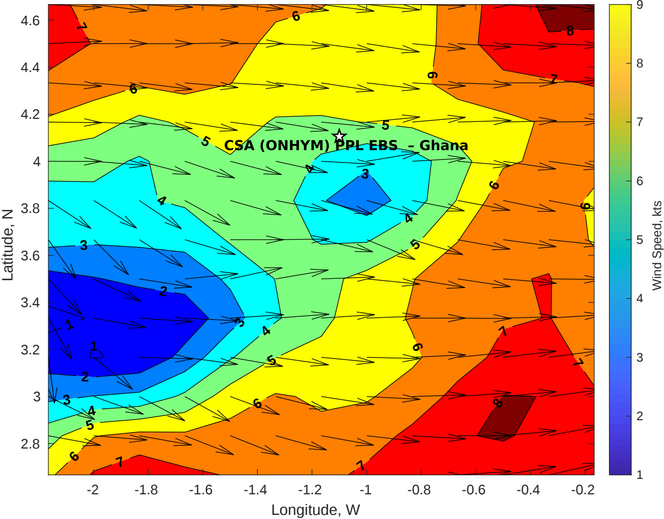
Winds (kts) for CSA (ONHYM) PPL EBS - Ghana at 02-May-2025 09:00:00
