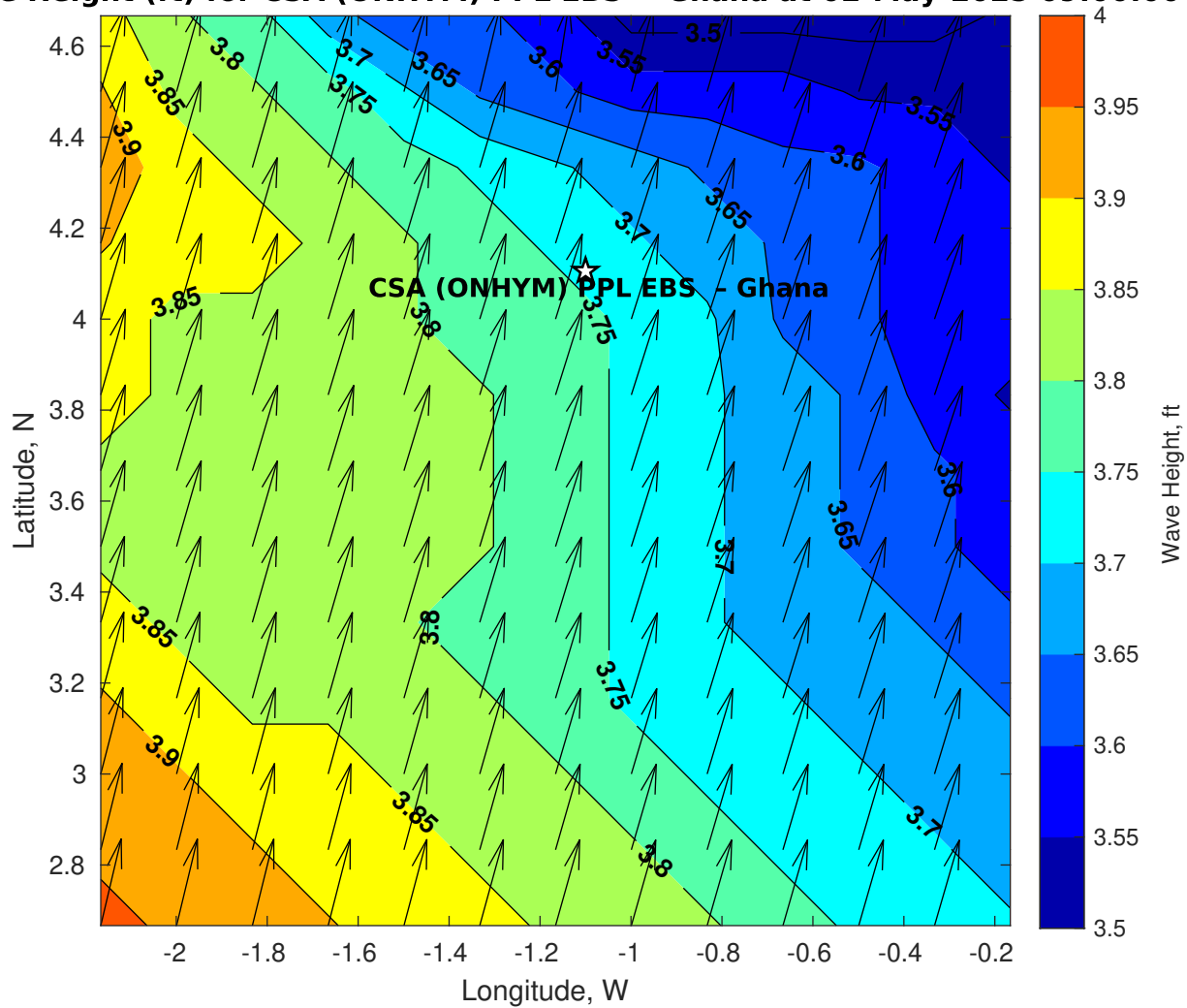
Wave Height (ft) for CSA (ONHYM) PPL EBS - Ghana at 02-May-2025 09:00:00
