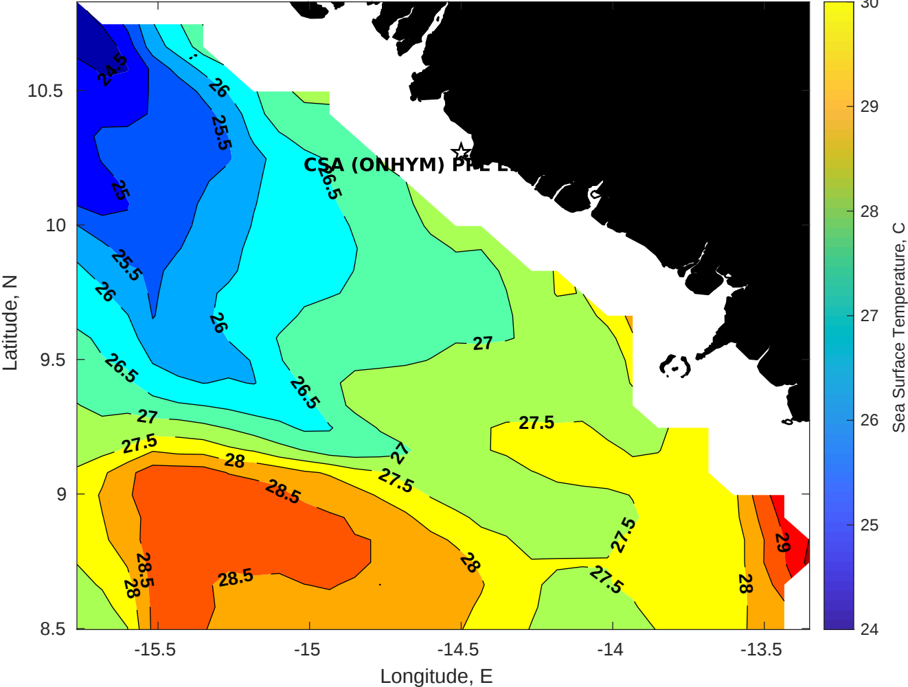
SST for CSA (ONHYM) PPL EBS - Guinea at 01-May-2025 00:00:00
