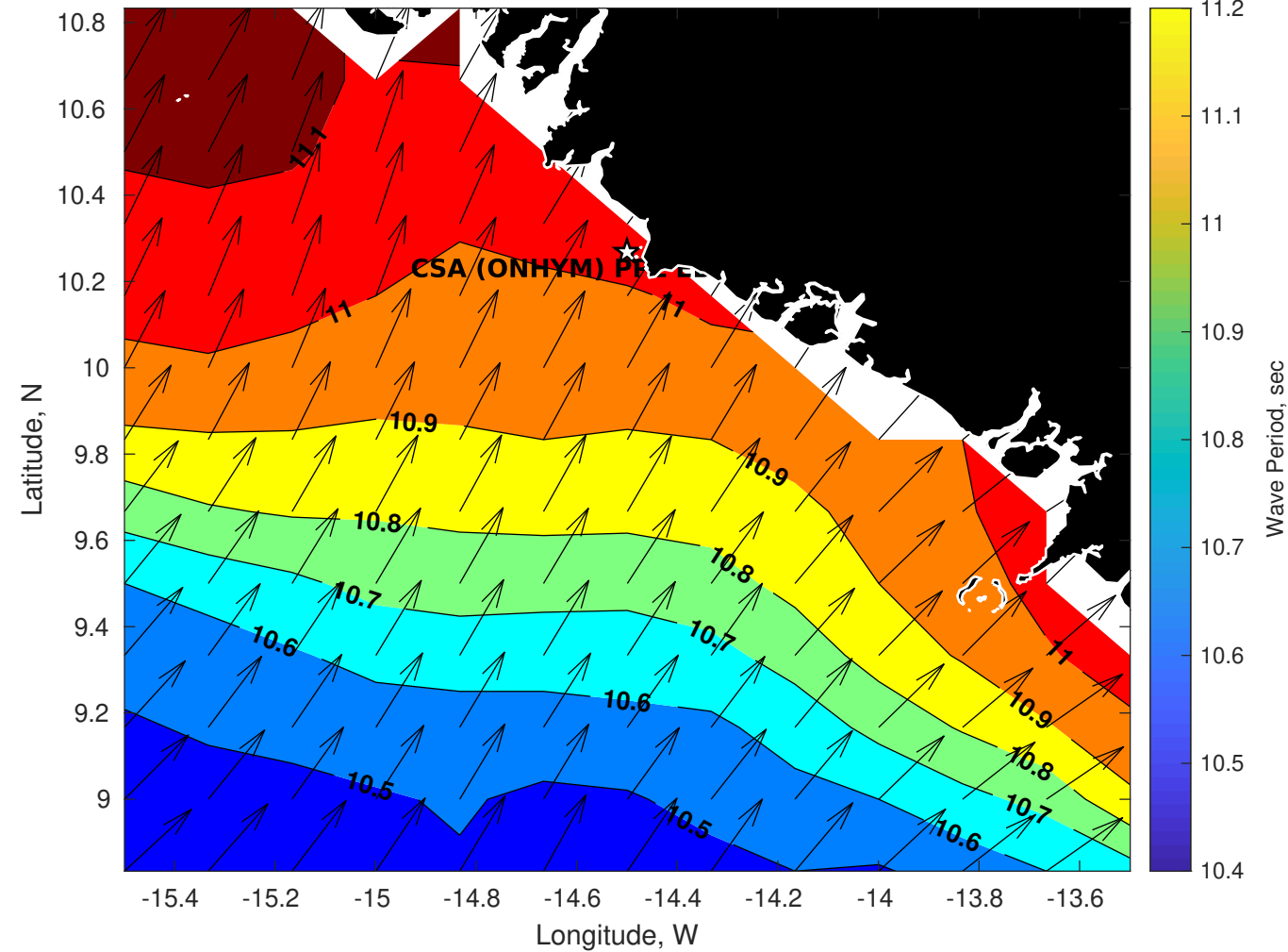
Wave Period (sec) for CSA (ONHYM) PPL EBS - Guinea at 02-May-2025 09:00:00
