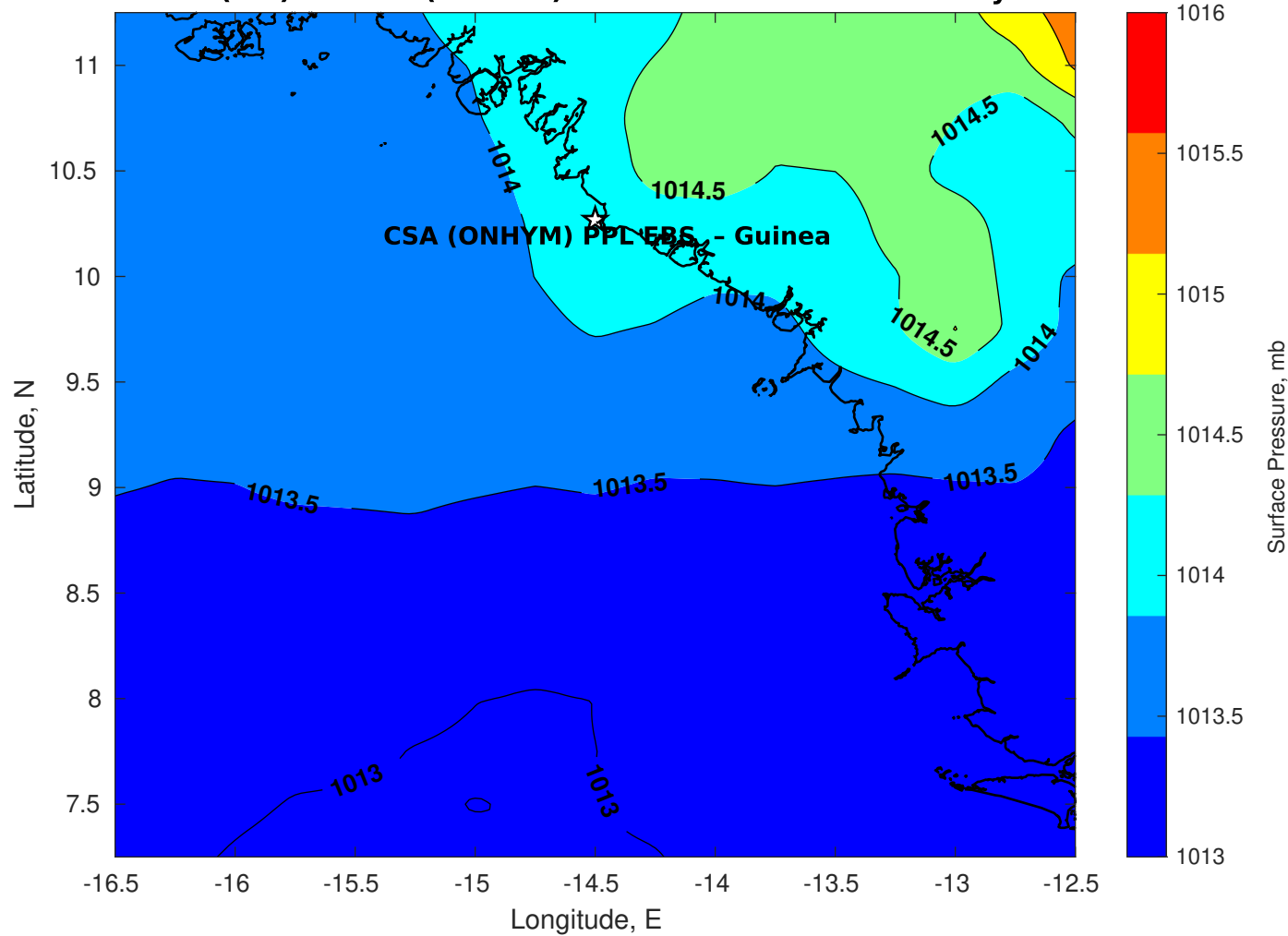
Surface Pressure (mb) for CSA (ONHYM) PPL EBS - Guinea at 03-May-2025 00:00:00
