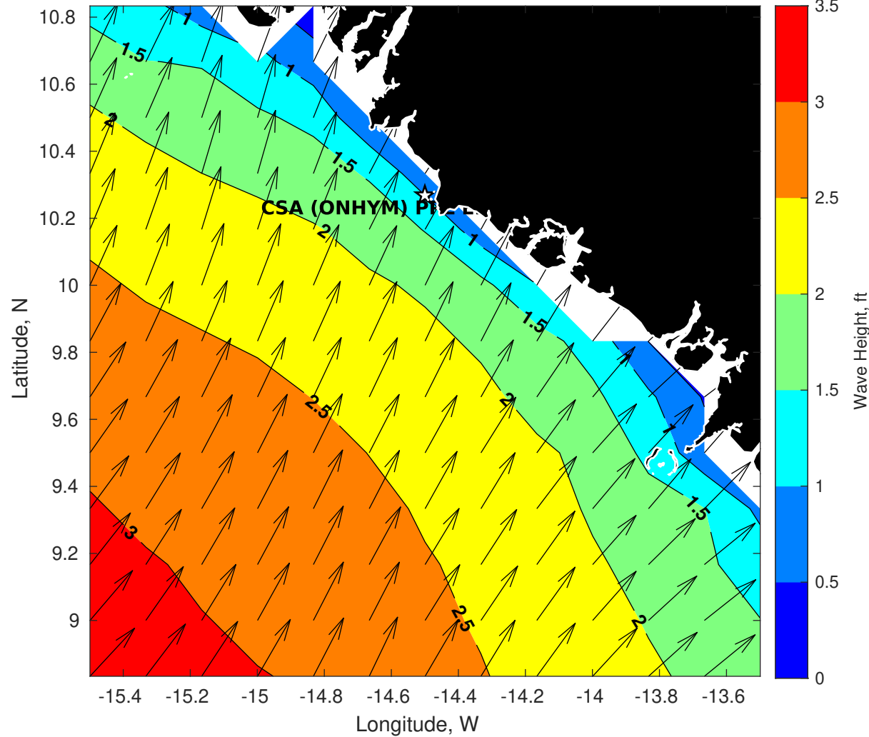
Wave Height (ft) for CSA (ONHYM) PPL EBS - Guinea at 02-May-2025 09:00:00
