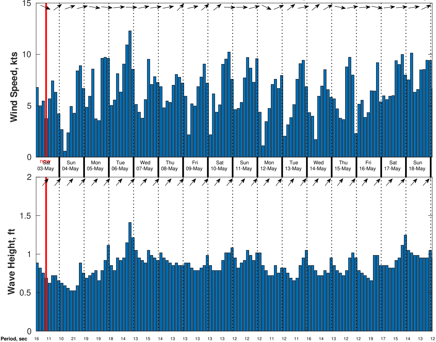
Wind & Wave Forecast for CSA (ONHYM) PPL EBS - Guinea from 02-May-2025 01:00:00 to 18-May-2025 01:00:00
