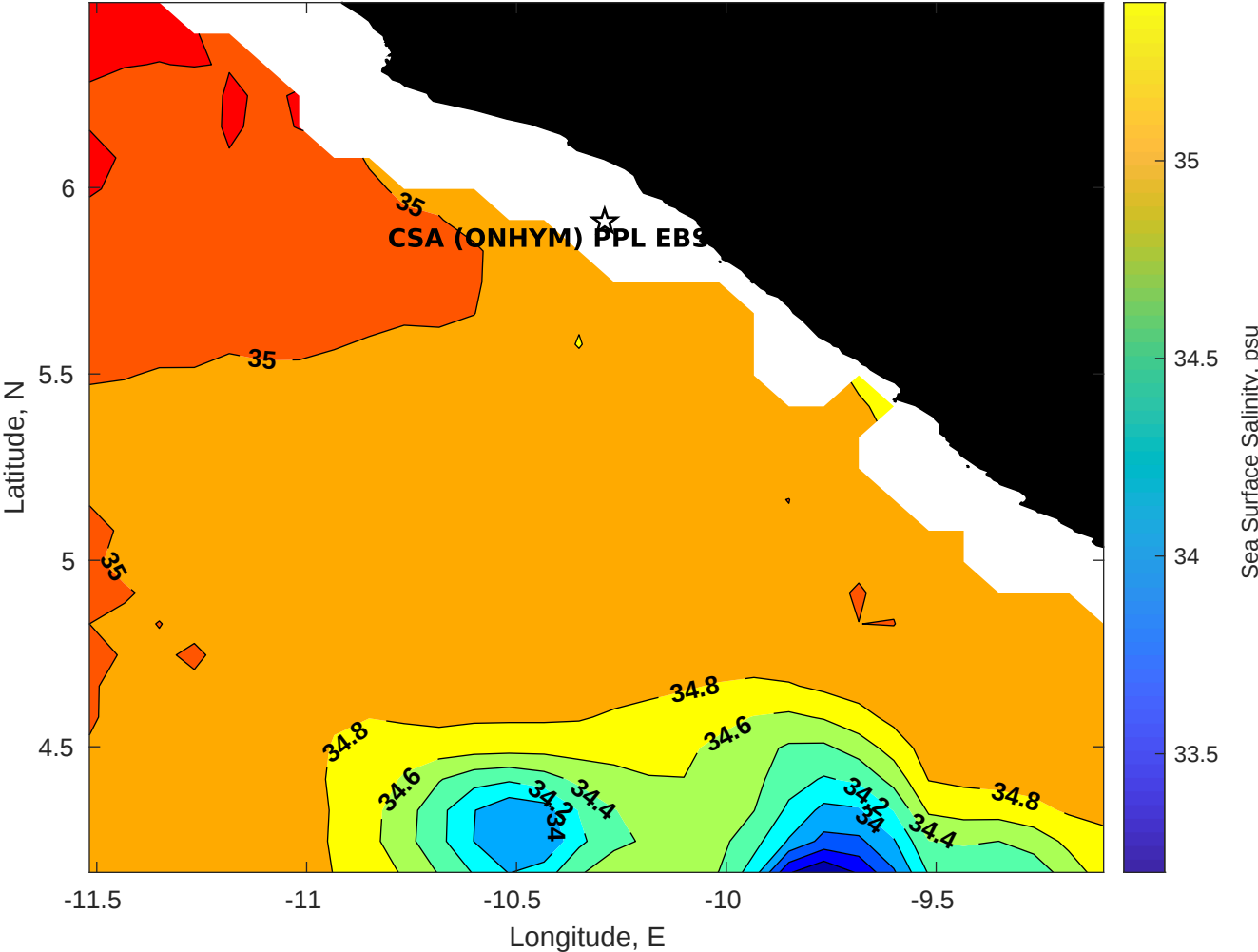
Surface Salinity for CSA (ONHYM) PPL EBS - Liberia at 01-May-2025 00:00:00
