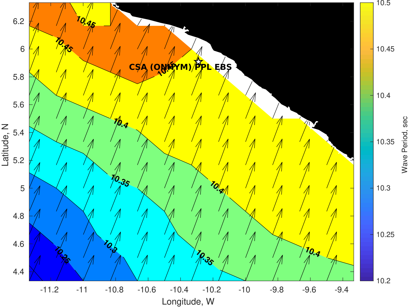
Wave Period (sec) for CSA (ONHYM) PPL EBS - Liberia at 02-May-2025 09:00:00
