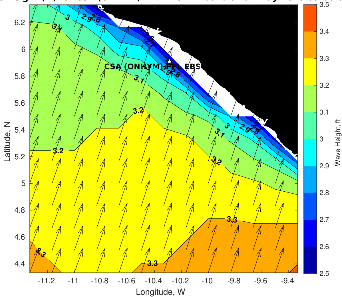
Wave Height (ft) for CSA (ONHYM) PPL EBS - Liberia at 02-May-2025 09:00:00
