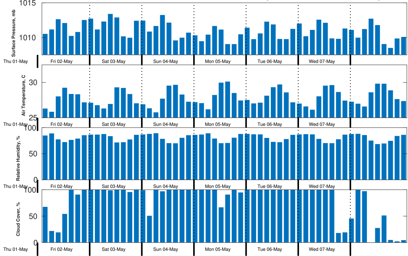
Met Forecast for CSA (ONHYM) PPL EBS - Liberia from 02-May-2025 00:00:00 to 09-May-2025 00:00:00
