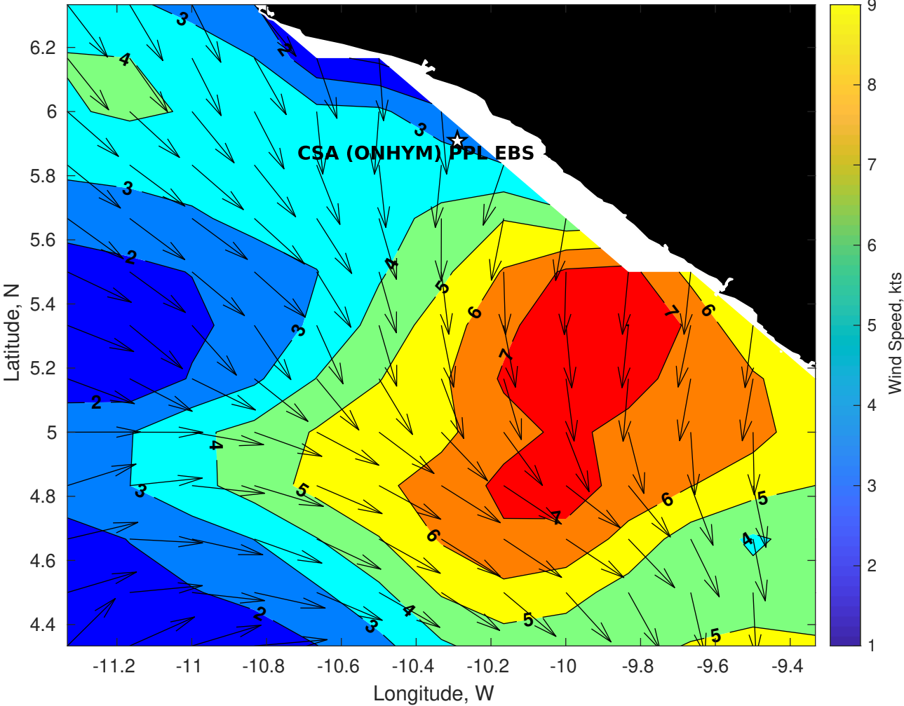
Winds (kts) for CSA (ONHYM) PPL EBS - Liberia at 02-May-2025 09:00:00
