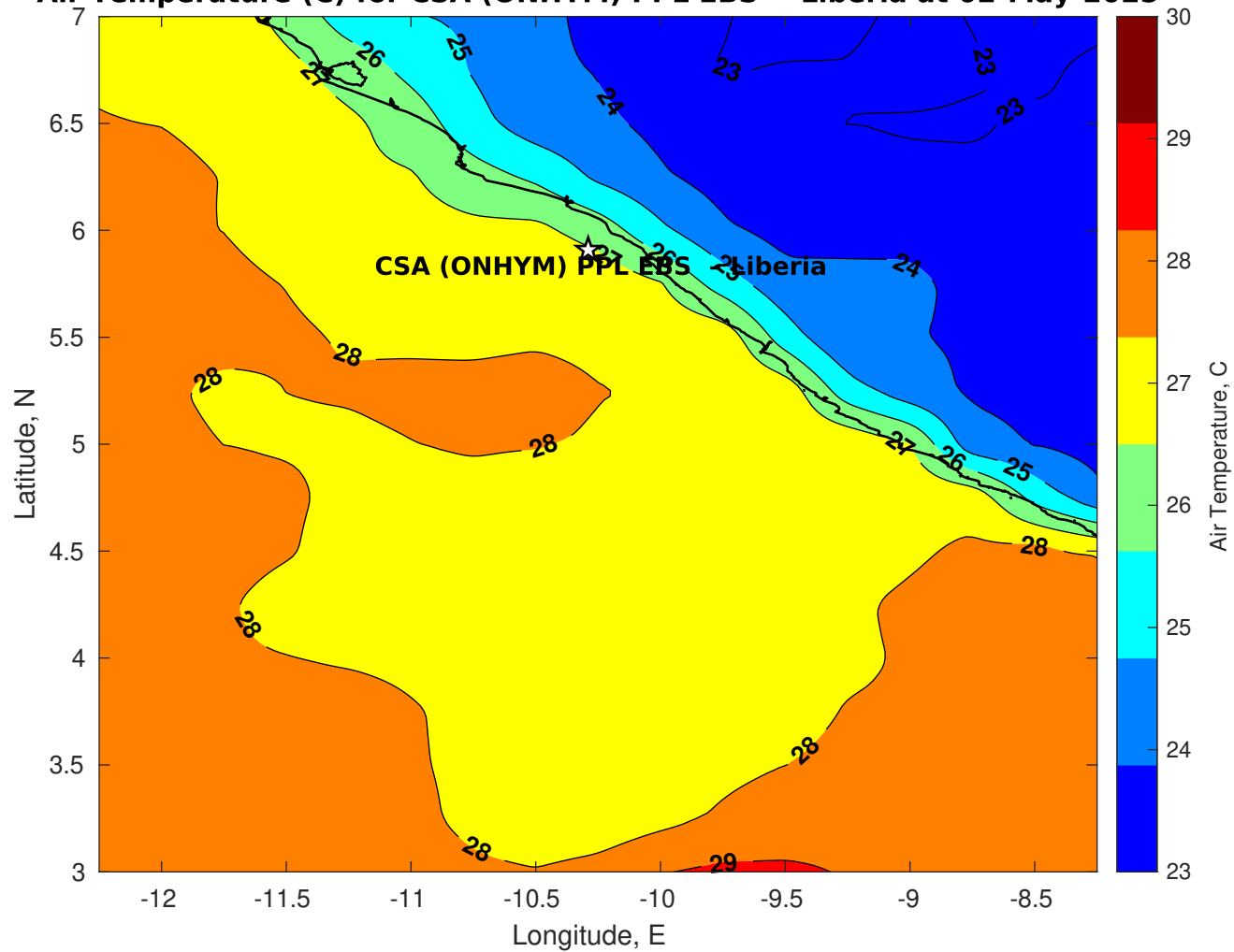
Air Temperature (C) for CSA (ONHYM) PPL EBS - Liberia at 02-May-2025
