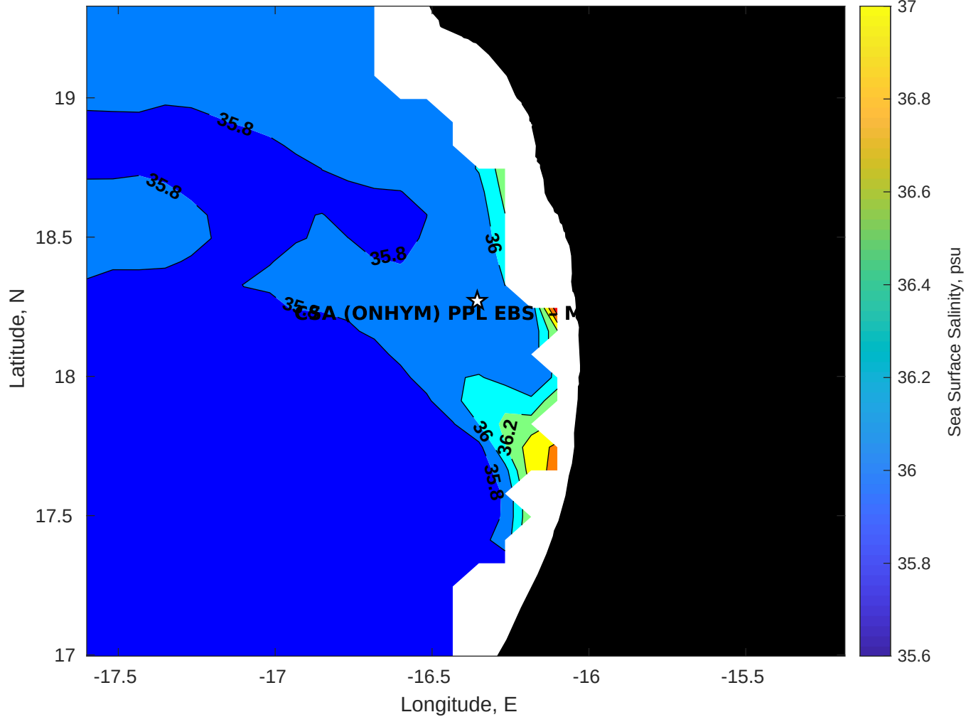
Surface Salinity for CSA (ONHYM) PPL EBS - Mauritania at 01-May-2025 00:00:00
