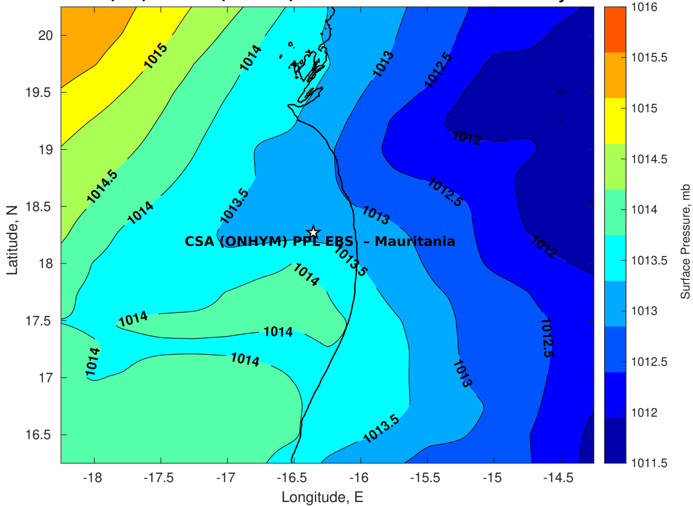
Surface Pressure (mb) for CSA (ONHYM) PPL EBS - Mauritania at 04-May-2025 00:00:00
