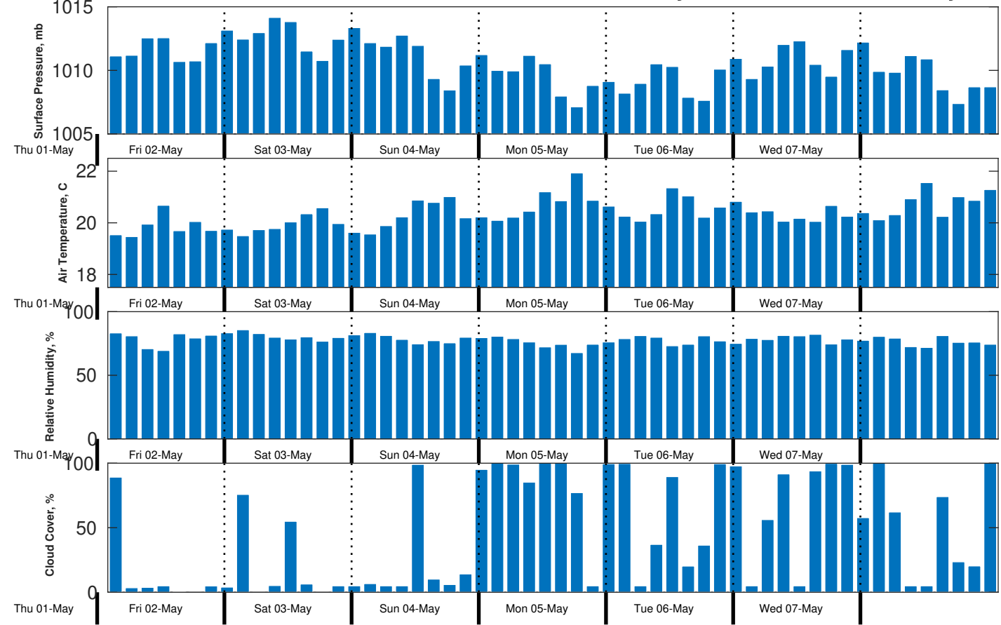
Met Forecast for CSA (ONHYM) PPL EBS - Mauritania from 02-May-2025 00:00:00 to 09-May-2025 00:00:00
