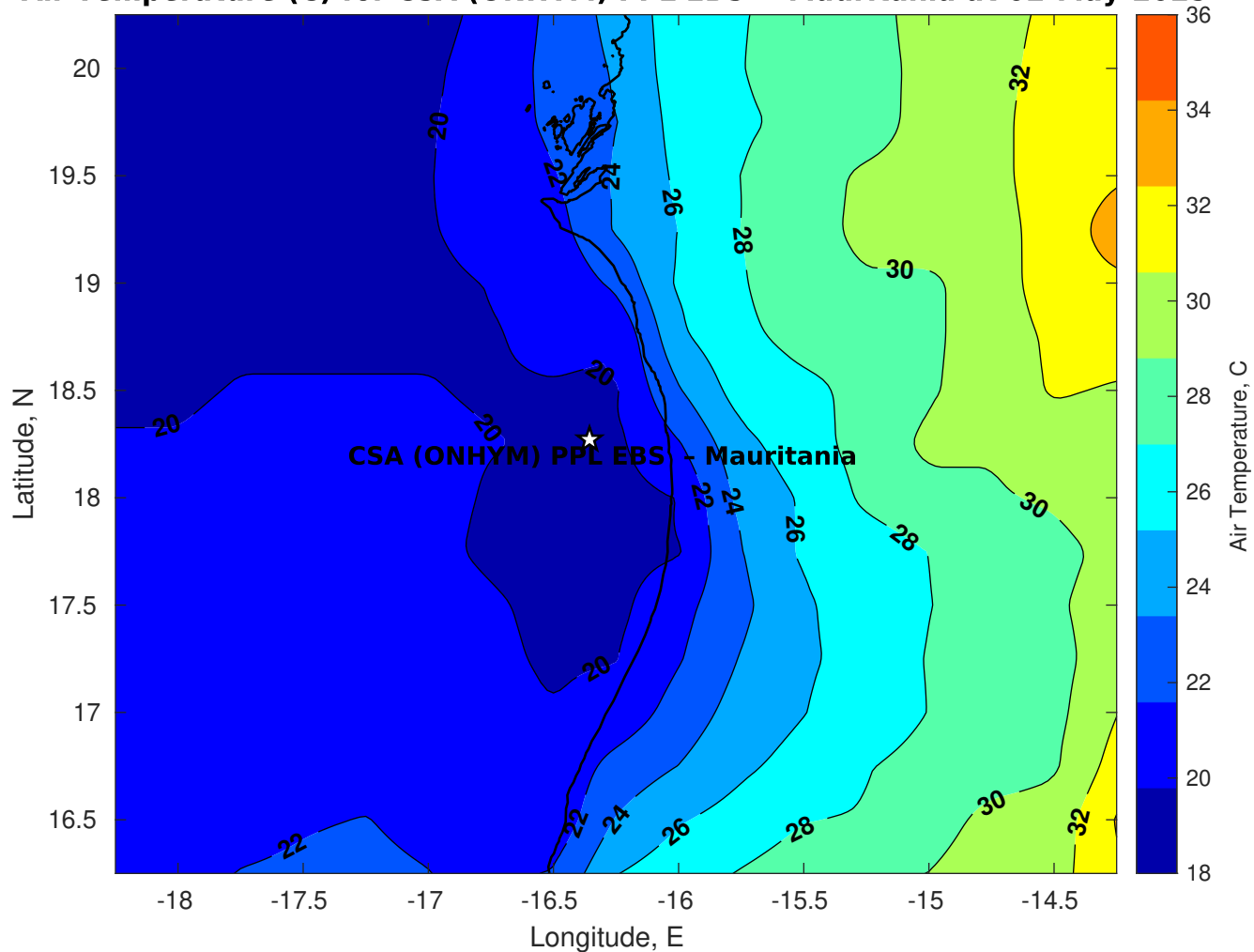
Air Temperature (C) for CSA (ONHYM) PPL EBS - Mauritania at 02-May-2025
