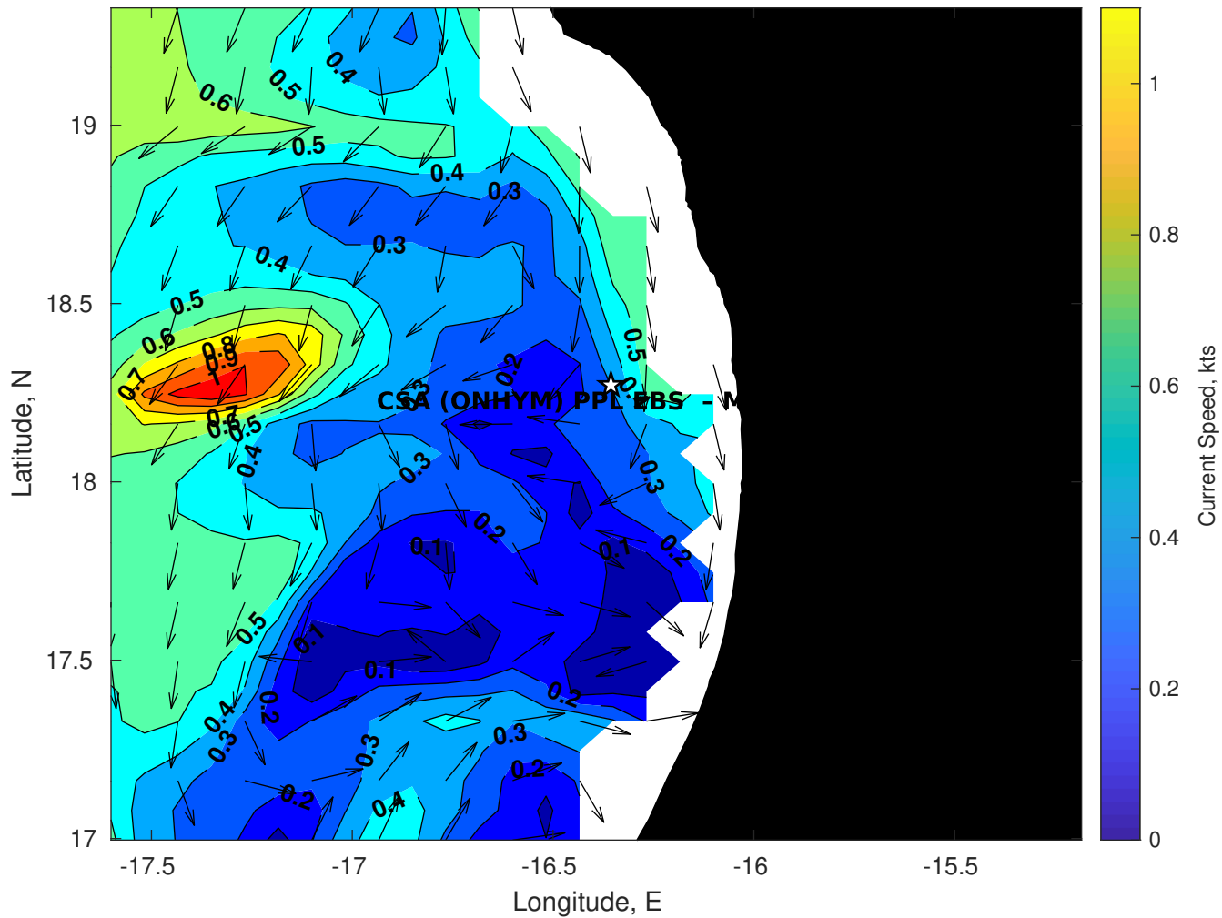
Surface Currents for CSA (ONHYM) PPL EBS - Mauritania at 01-May-2025 00:00:00
