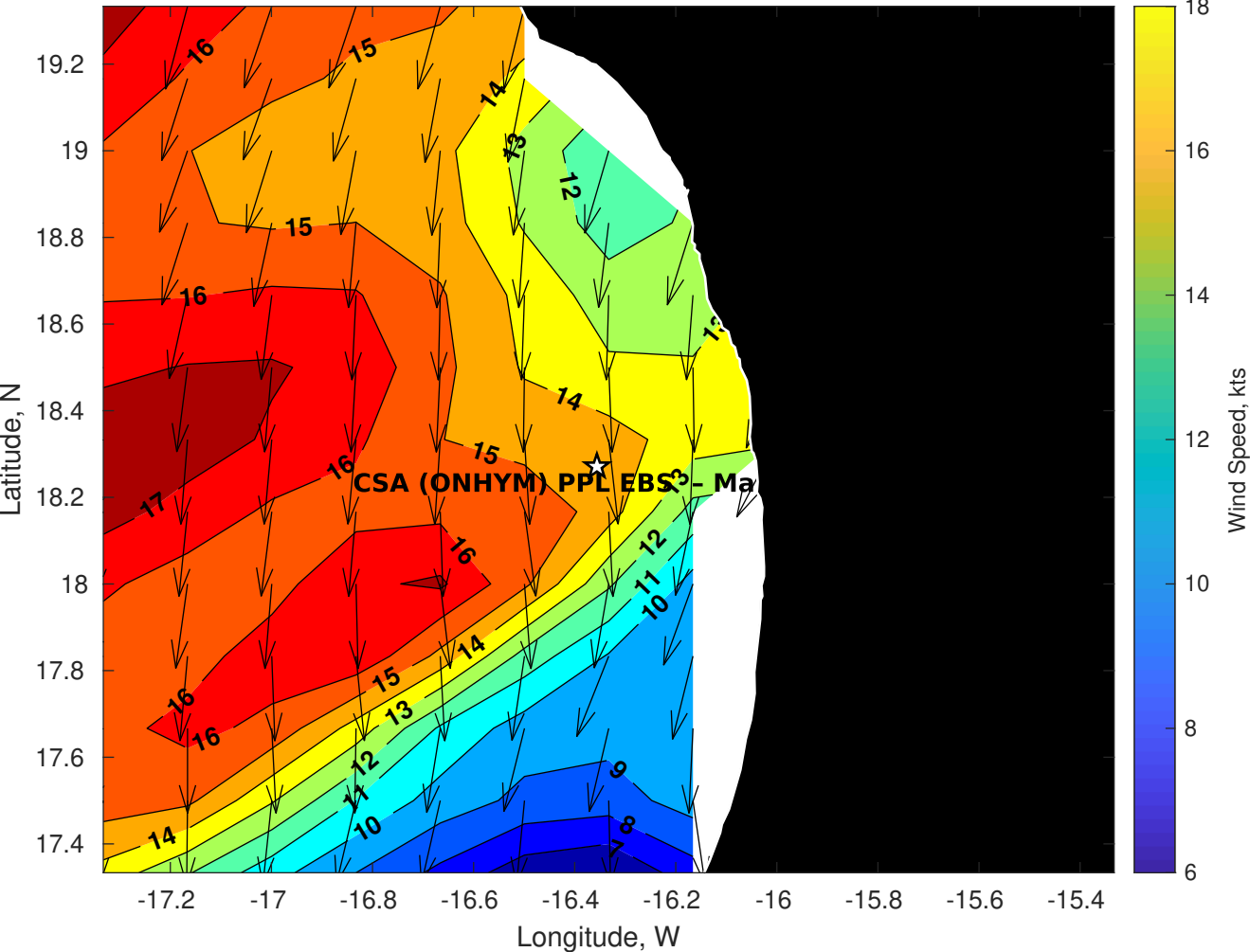
Winds (kts) for CSA (ONHYM) PPL EBS - Mauritania at 02-May-2025 09:00:00
