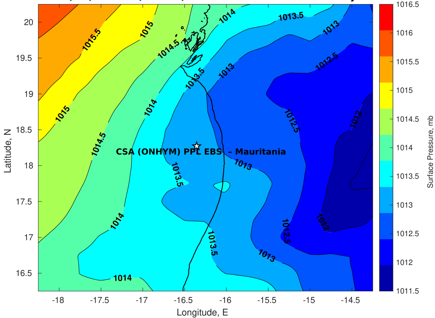
Surface Pressure (mb) for CSA (ONHYM) PPL EBS - Mauritania at 03-May-2025 00:00:00
