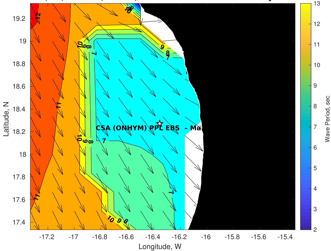
Wave Period (sec) for CSA (ONHYM) PPL EBS - Mauritania at 02-May-2025 09:00:00
