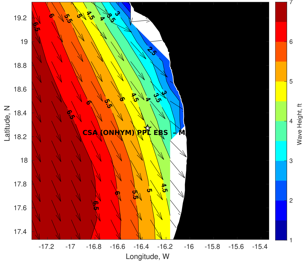
Wave Height (ft) for CSA (ONHYM) PPL EBS - Mauritania at 02-May-2025 09:00:00
