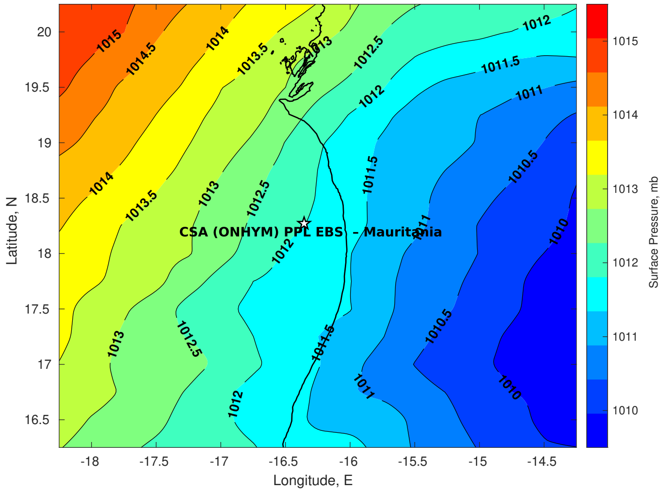
Surface Pressure (mb) for CSA (ONHYM) PPL EBS - Mauritania at 02-May-2025 00:00:00
