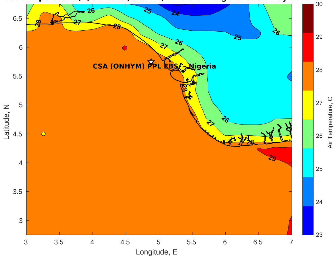
Air Temperature (C) for CSA (ONHYM) PPL EBS - Nigeria at 02-May-2025
